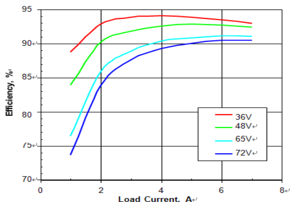
Figure 2. Efficiency vs. load current and input voltage for SSQE48S07120 converter mounted vertically with air flowing from pin 1 to pin 3 at a rate of 300 LFM (1.5m/s) and T_a = 25^\circ C .
