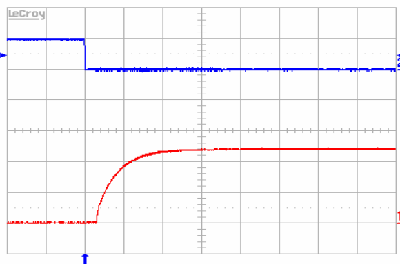
Figure 6. Turn-on transient at full rated load current (resistive) with no output capacitor at V_{in} = 48V , triggered via ON/OFF pin. Top trace: ON/OFF signal (5V/div.). Bottom trace: Output voltage (5V/div.). Time scale: 2ms/div.
