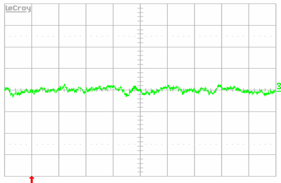
Figure 12. Input reflected-ripple current, i_s (10mA/div.), measured through 10 \mu H at the source at full rated load current and V_{in} = 48V . Refer to Figure 11 for test setup. Time scale: 1 \mu s/div.
