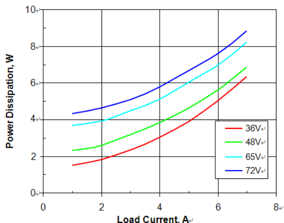
Figure 4. Power dissipation vs. load current and input voltage for SSQE48S07120 converter mounted vertically with air flowing from pin 1 to pin 3 at a rate of 300 LFM (1.5 m/s) and T_a = 25^\circ C .
