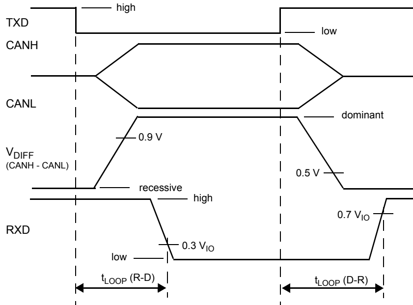
Figure 9. CAN Timing Diagram
