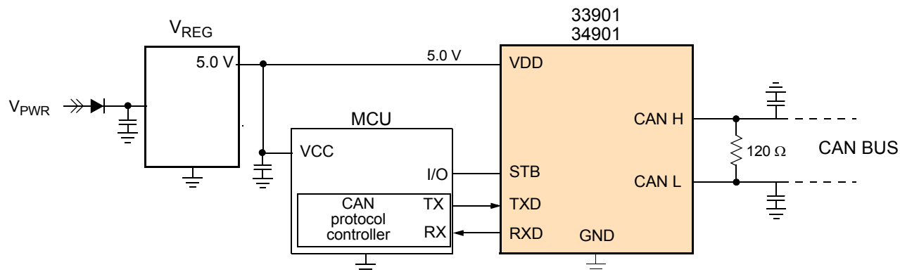
Figure 2. Simplified Application Diagram for MC3x901xNEF
