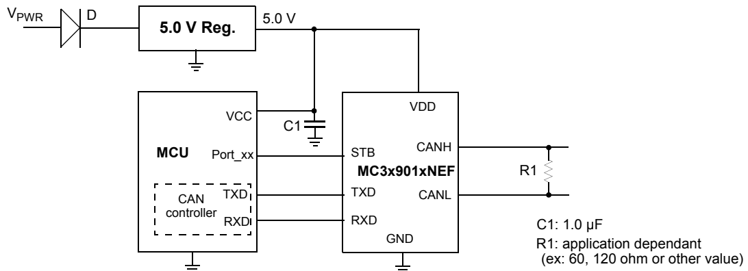
Figure 14. Single Supply Typical Application Schematic for MC3x901xNEF
