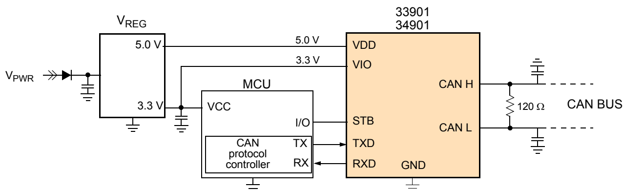
Figure 1. Simplified Application Diagram for MC3x901xEF
