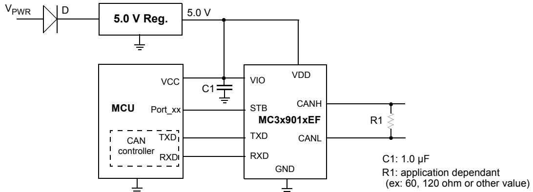
Figure 13. Single Supply Typical Application Schematic for MC3x901xEF
