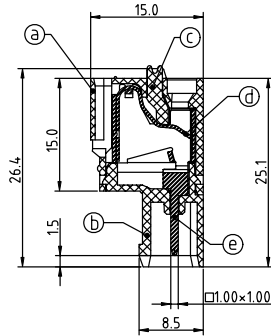
SECTION P-P
