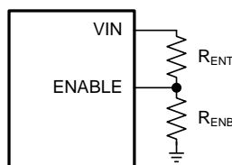
Figure 36. System UVLO By Enable Dividers
