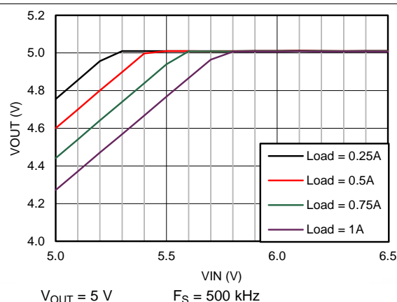
Figure 56. Drop-Out Curve
