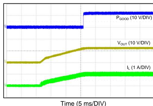
Figure 96. Startup with External Capacitor C_{SS} = 33\text{ nF}
