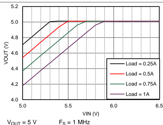
Figure 16. Drop-Out Curve
