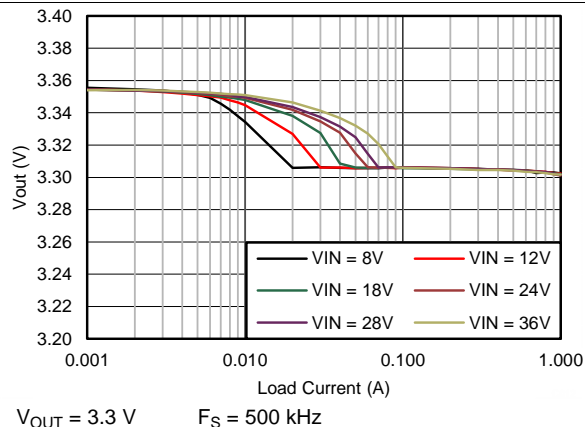
Figure 7. V_{OUT} Regulation
