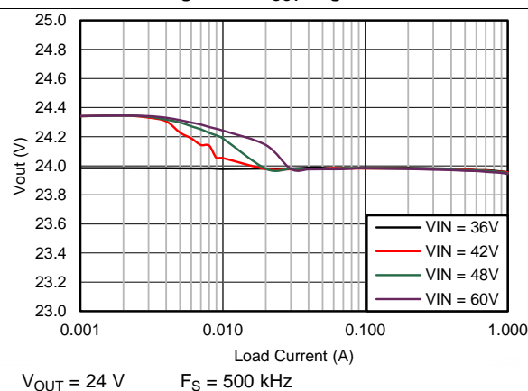
Figure 12. V_{OUT} Regulation
