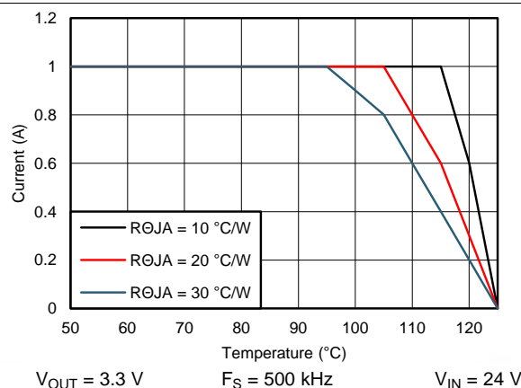
Figure 52. Derating Curve
