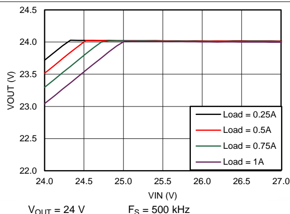
Figure 80. Drop-Out Curve
