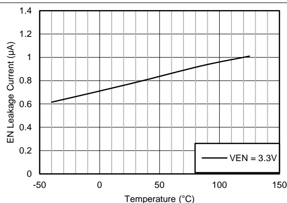
Figure 28. Enable Leakage Current vs Junction Temperature
