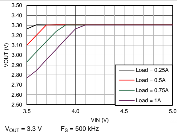
Figure 13. Drop-Out Curve
