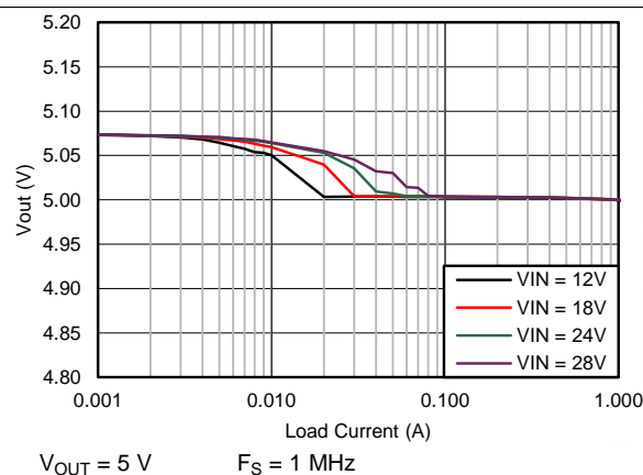
Figure 10. V_{OUT} Regulation
