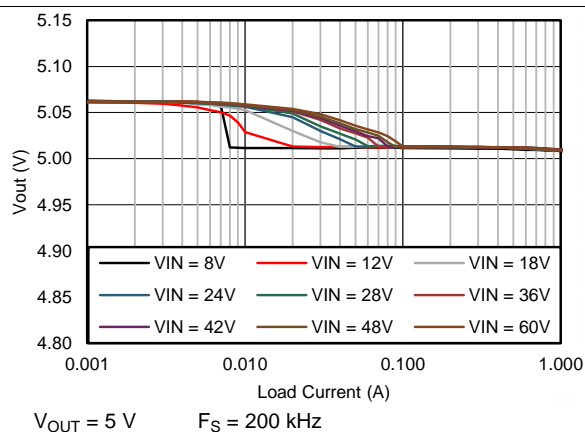
Figure 9. V_{OUT} Regulation
