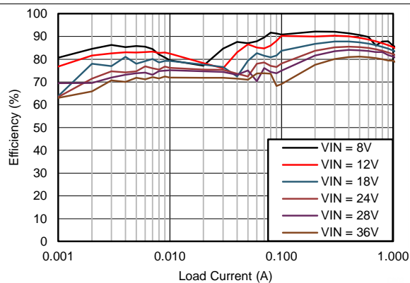
Figure 1. Efficiency
