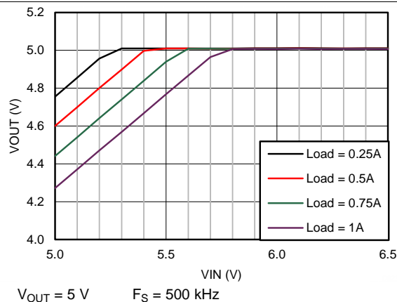
Figure 14. Drop-Out Curve
