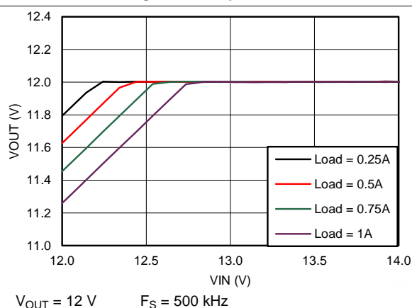
Figure 17. Drop-Out Curve
