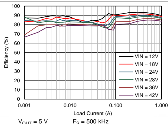
Figure 54. Efficiency
