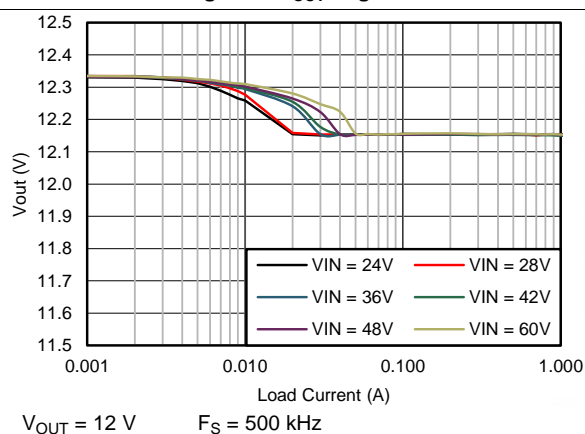
Figure 11. V_{OUT} Regulation
