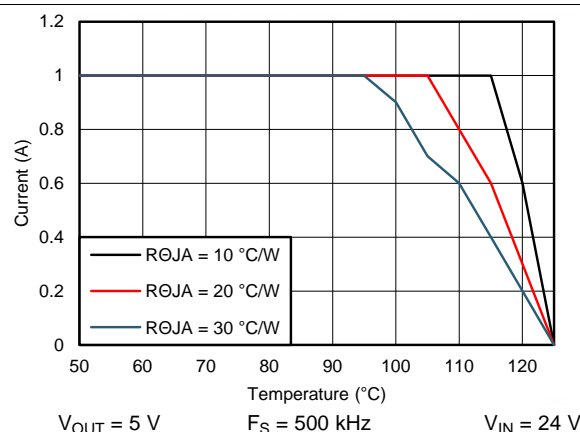
Figure 58. Derating Curve
