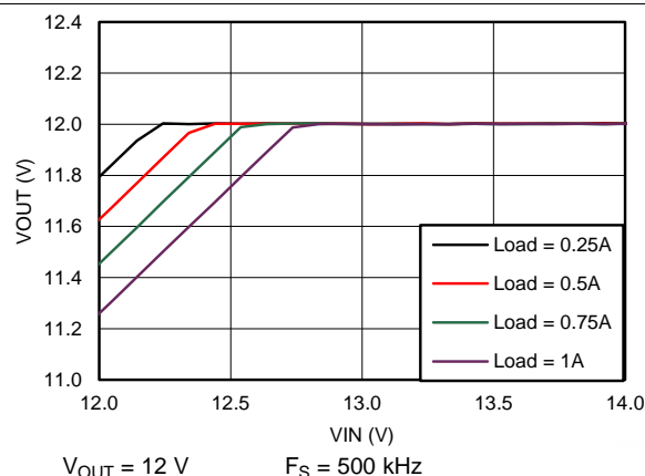
Figure 74. Drop-Out Curve
