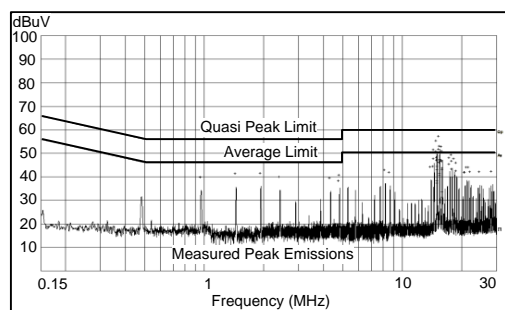
V_{OUT} = 3.3\text{ V} F_S = 500\text{ kHz} I_{OUT} = 1\text{ A} Measured on the LM46001PWPEVM with default BOM. EVM input filter: L_{in} = 1\text{ }\mu\text{H} C_d = 47\text{ }\mu\text{F} C_{IN4} = 68\text{ }\mu\text{F}
