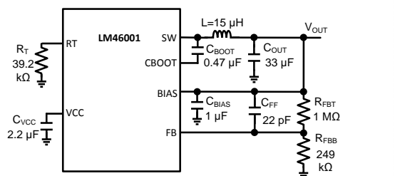
Figure 65. BOM for V_{OUT} = 5\text{ V} , F_S = 1\text{ MHz}
