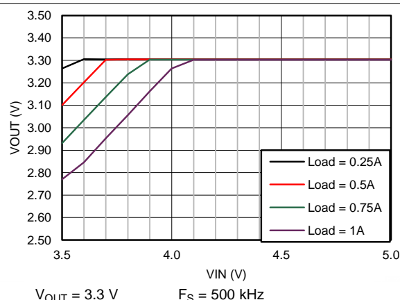
Figure 50. Drop-Out Curve
