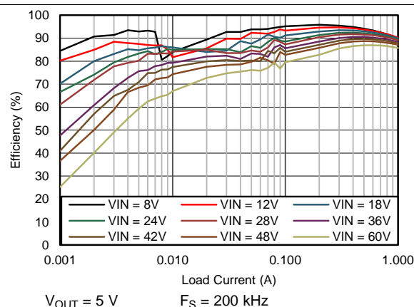
Figure 60. Efficiency
