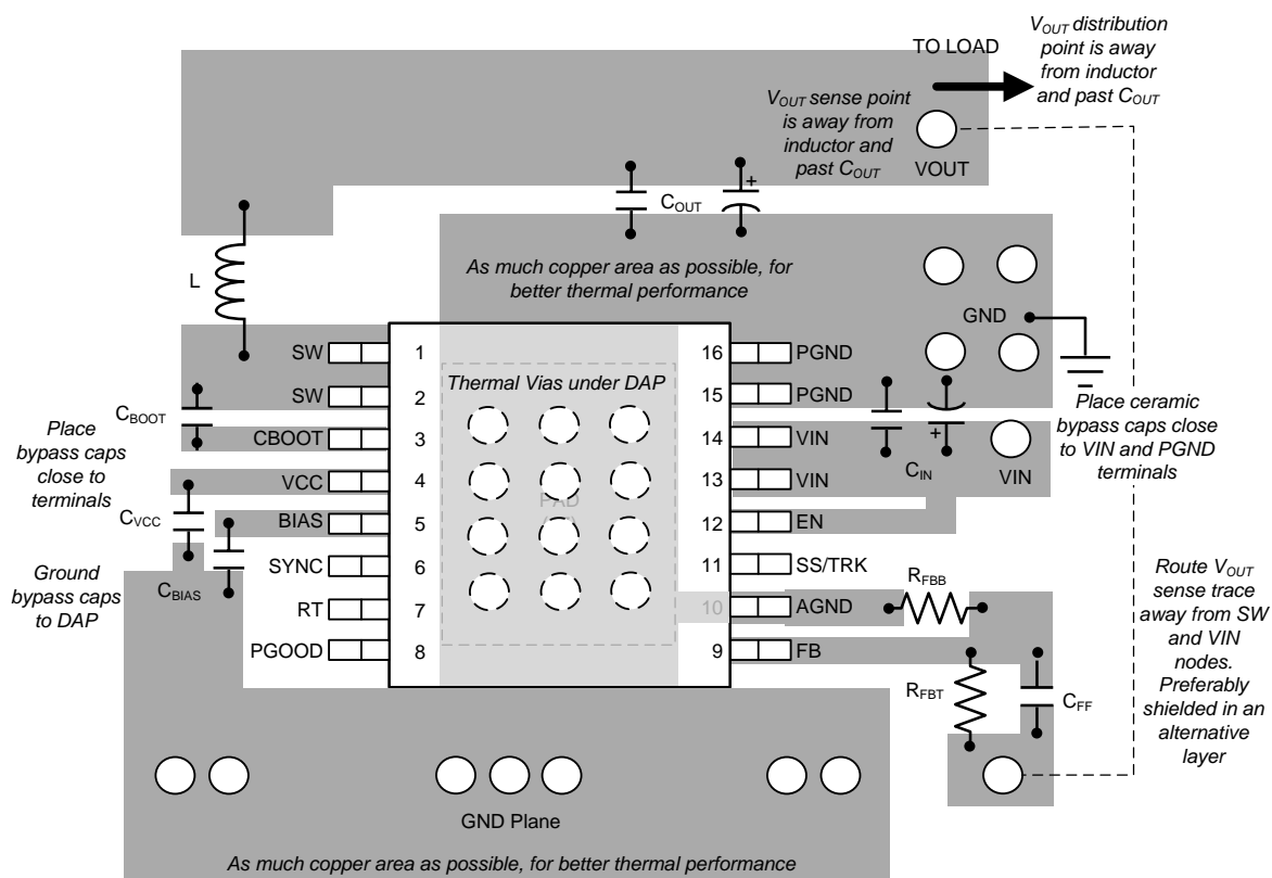
Figure 102. LM46001 PCB Layout Example
