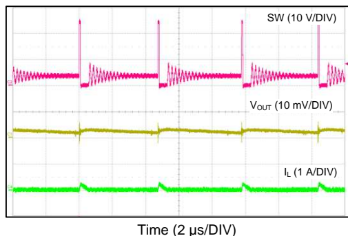
Figure 89. Switching Waveform in CCM Operation
