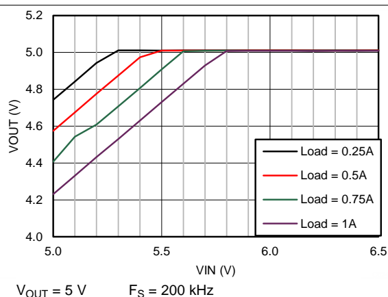
Figure 15. Drop-Out Curve
