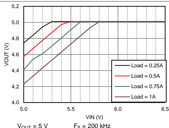
Figure 62. Drop-Out Curve
