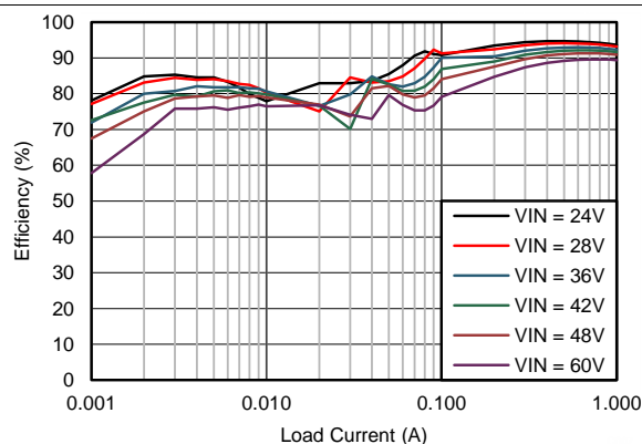
Figure 3. Efficiency
