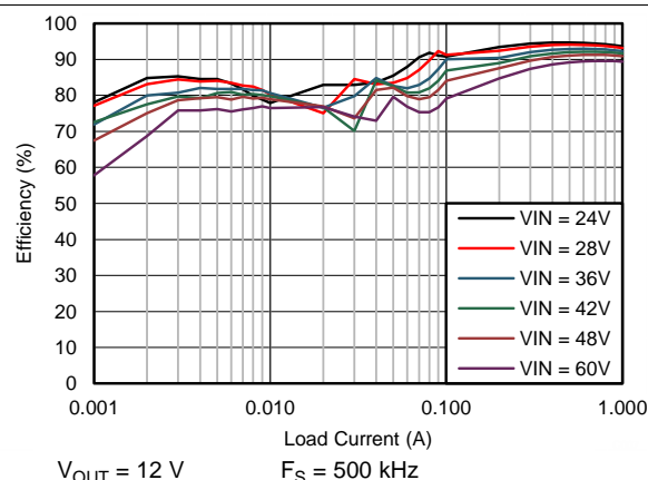
Figure 72. Efficiency
