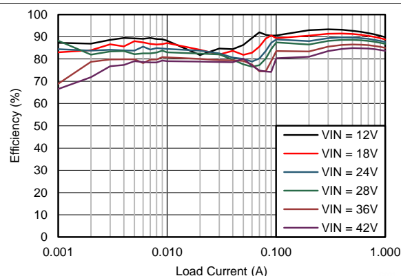
Figure 2. Efficiency
