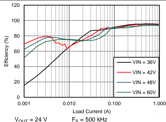
Figure 78. Efficiency
