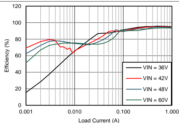
Figure 4. Efficiency
