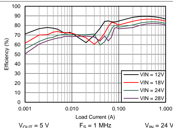
Figure 66. Efficiency
