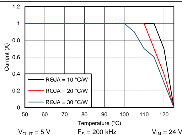
Figure 64. Derating Curve
