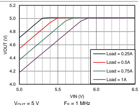
Figure 68. Drop-Out Curve
