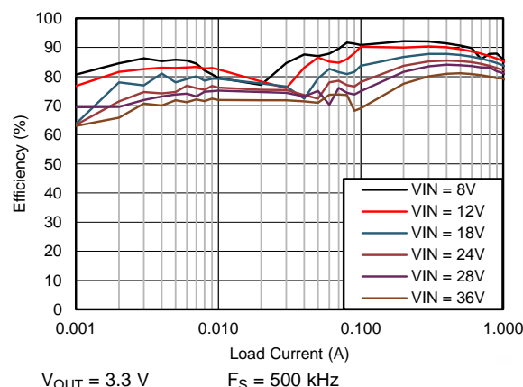
Figure 48. Efficiency
