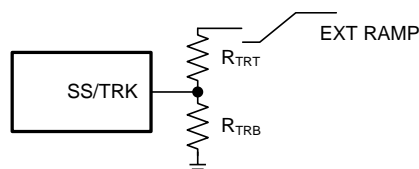
Figure 37. Soft Start Tracking External Ramp
