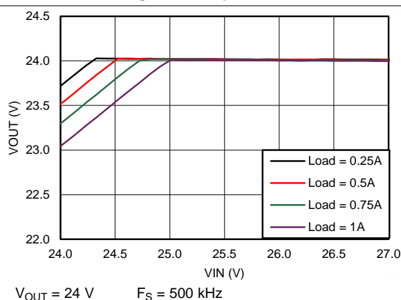
Figure 18. Drop-Out Curve
