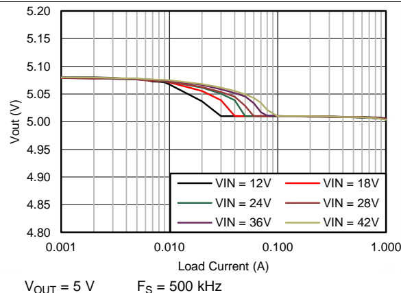
Figure 8. V_{OUT} Regulation
