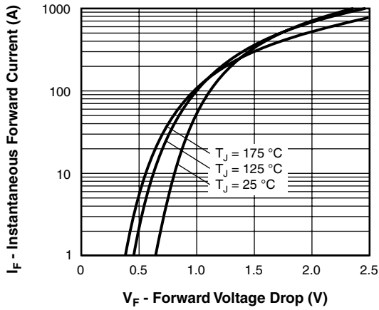
Fig. 1 - Typical Forward Voltage Drop Characteristics (Per Diode)
