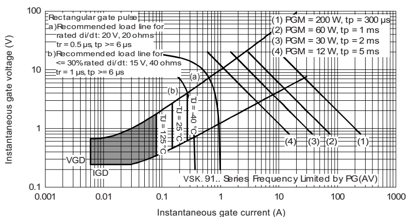
Fig. 12 - Gate Characteristics
