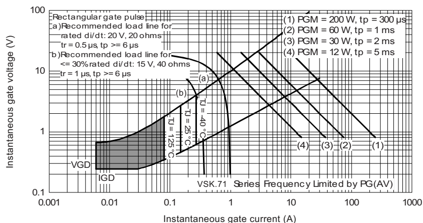
Fig. 11 - Gate Characteristics
