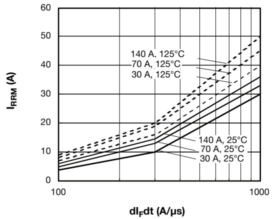
Fig. 6 - Typical Recovery Current vs. dI/dt (Per Leg)
