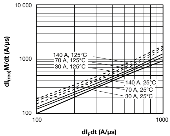
Fig. 8 - Typical dI_{(rec)}M/dt vs. dI/dt (Per Leg)
