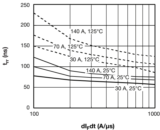
Fig. 5 - Typical Reverse Recovery Time vs. dI/dt (Per Leg)
