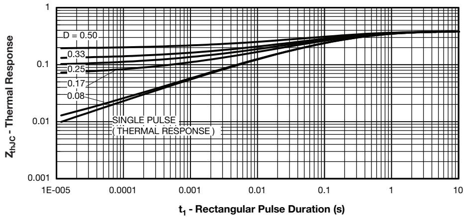
Fig. 9 - Maximum Thermal Impedance Z_{thJC} Characteristics
