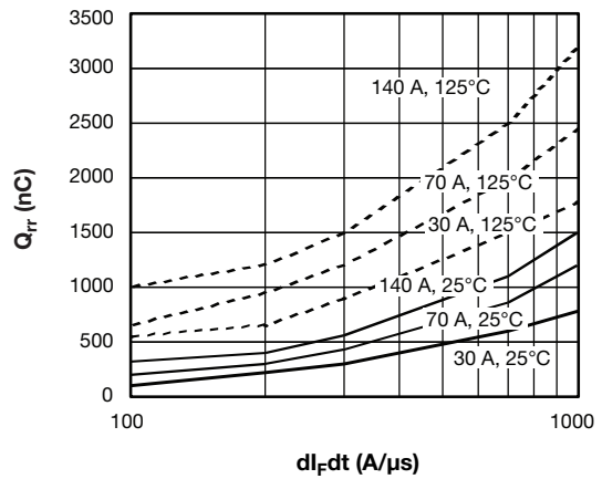
Fig. 7 - Typical Stored Charge vs. dI/dt (Per Leg)
