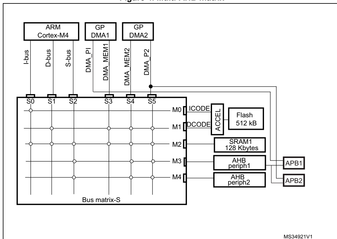
Figure 4. Multi-AHB matrix
