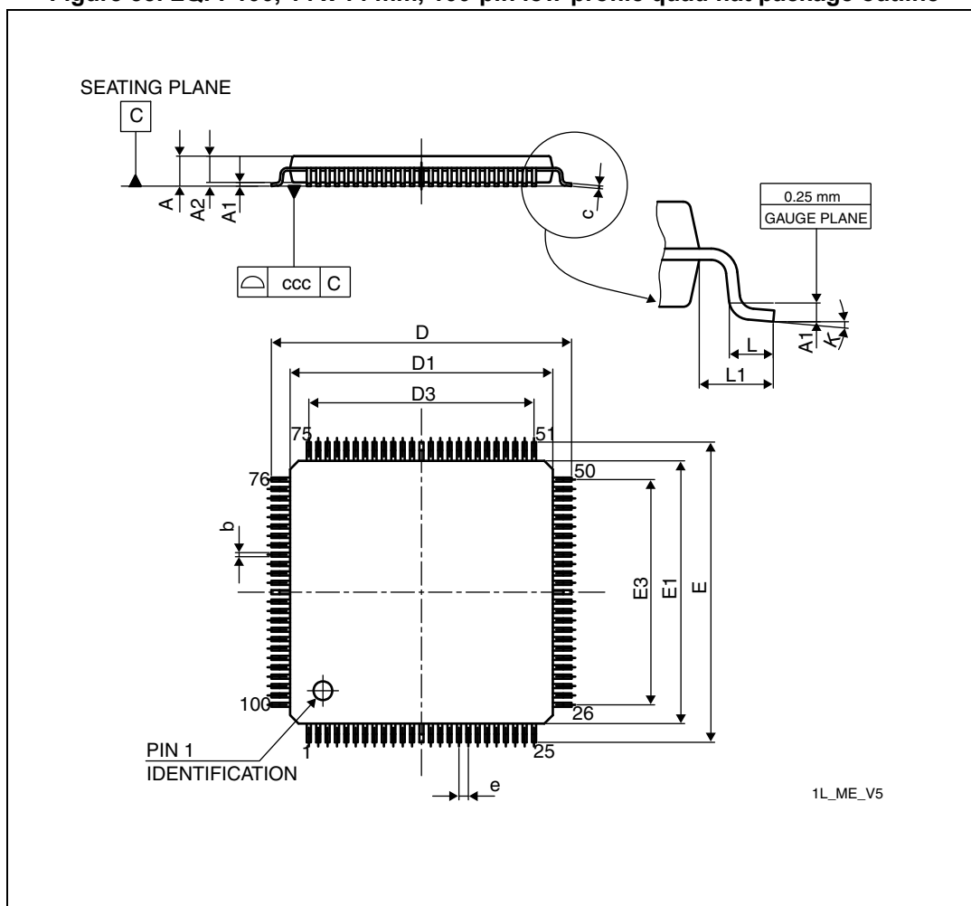
Figure 55. LQFP100, 14 x 14 mm, 100-pin low-profile quad flat package outline
