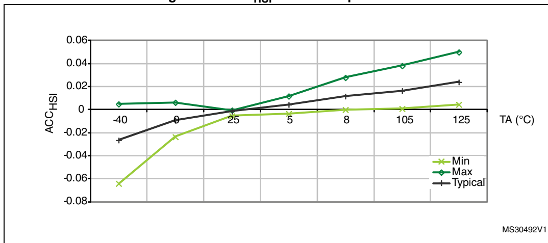
Figure 26. ACC HSI versus temperature
