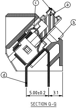
SECTION Q-Q
