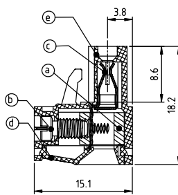
Section P-P
