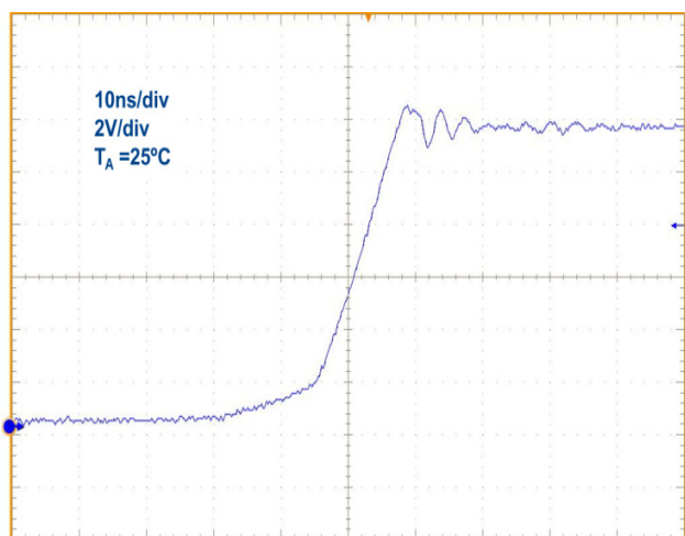
Figure 11 SW Output Rise Time
