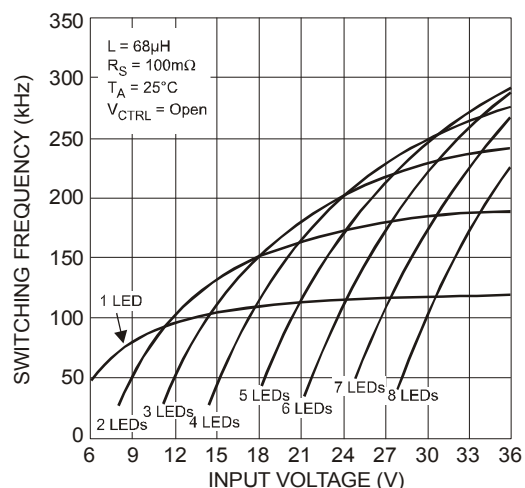
Figure 22. Switching Frequency vs. Input Voltage
