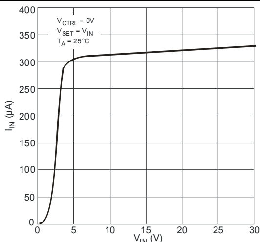
Supply Current (not switching) vs. Input Current
