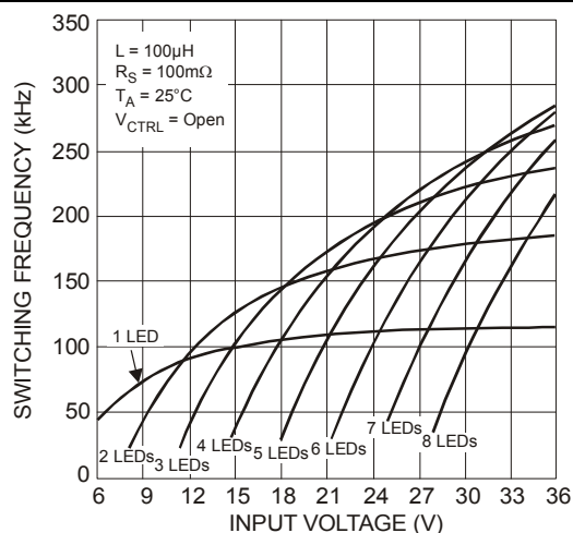
Figure 20. Switching Frequency vs. Input Voltage
