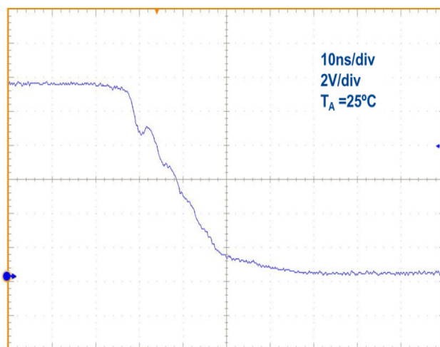
Figure 12 SW Output Fall Time
