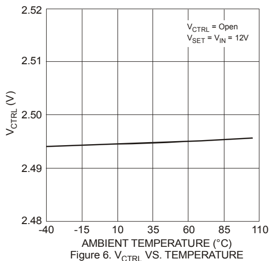
Figure 6. V_{CTRL} VS. TEMPERATURE
