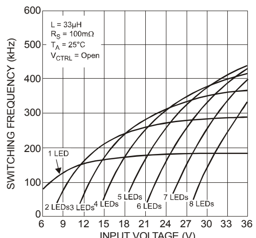
Figure 24. Switching Frequency vs. Input Voltage
