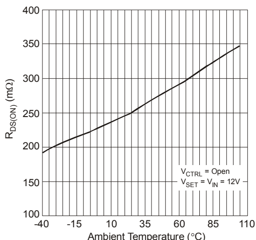
Figure 9. SW R_{DS(ON)} vs. Temperature
