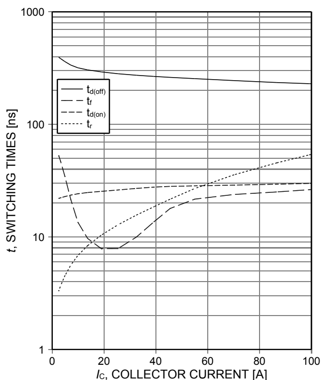
Figure 8. Typical switching times as a function of collector current (inductive load, T_{vj}=175^{\circ}\text{C} , V_{CE}=400\text{V} , V_{GE}=15\text{V} , R_{DS(on)}=80\text{m}\Omega , R_{DS(dynamic)}=80\text{m}\Omega )
