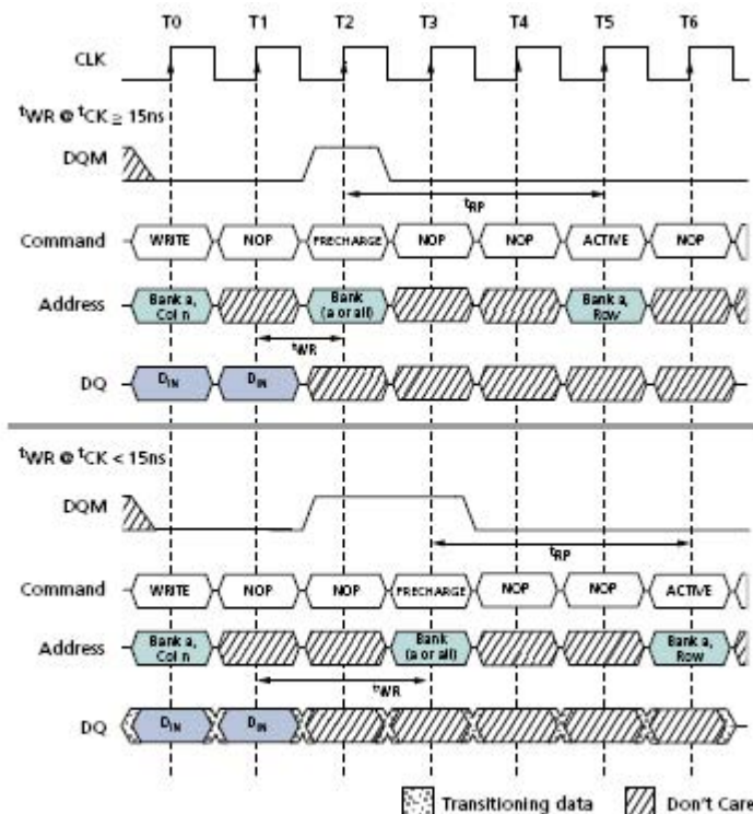
Figure 28: WRITE-to-PRECHARGE
