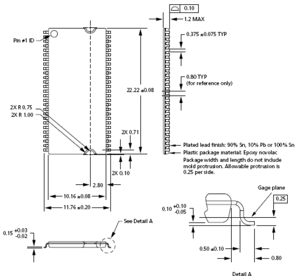
Figure 5: 54-Pin Plastic TSOP (400 mil) – Package Codes T
