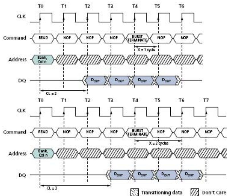
Figure 20: Terminating a READ Burst
