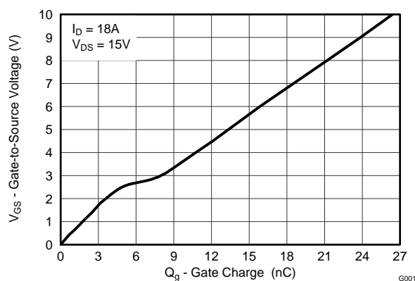
Gate Charge
