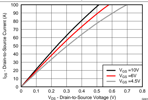
Figure 2. Saturation Characteristics
