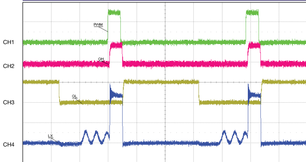
Fig. 8 - PS2 Mode Operation (ZCD) CH1 (green) = PWM (2V/div), CH2 (red) = GH (5V/div), CH3 (yellow) = GL (5V/div), CH4 (blue) = V_{SWH} (5V/div)
