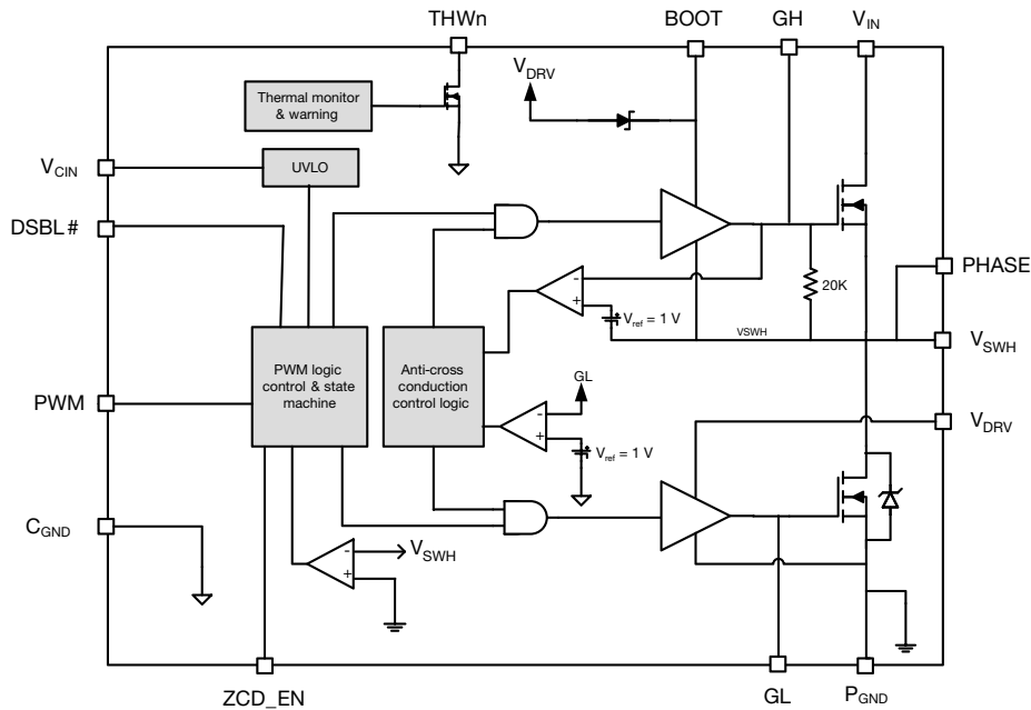
Fig. 4 - SiC781 Functional Block Diagram
