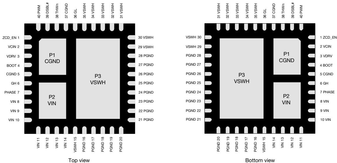
Fig. 2 - SiC781 Pin Configuration
