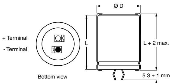
Fig. 2 - Two terminal snap-in
