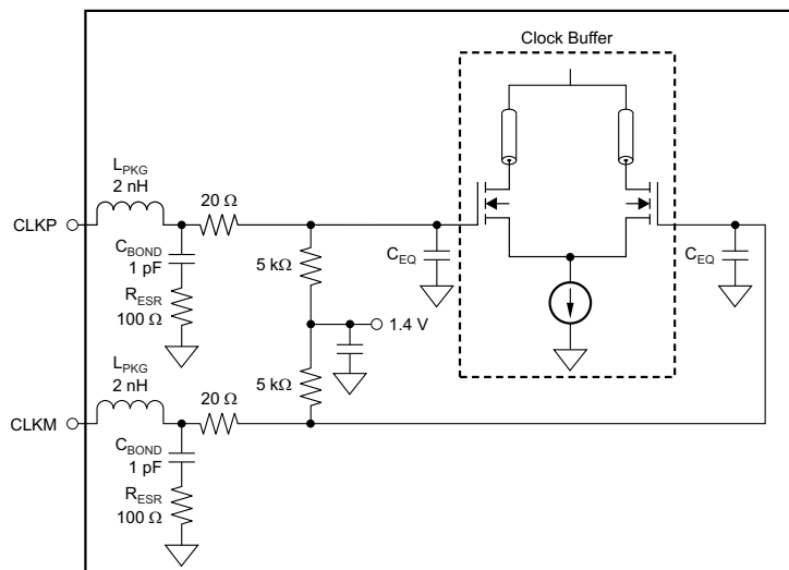
Figure 151. Internal Clock Buffer
