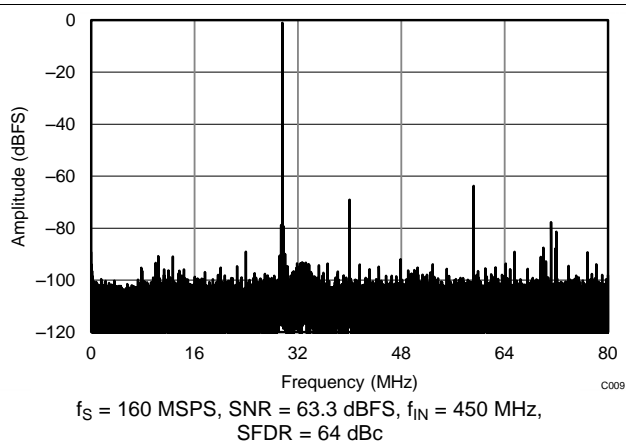
Figure 9. FFT for 450-MHz Input Signal, Dither On
