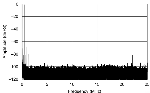
Figure 106. FFT for 270-MHz Input Signal, Dither On
