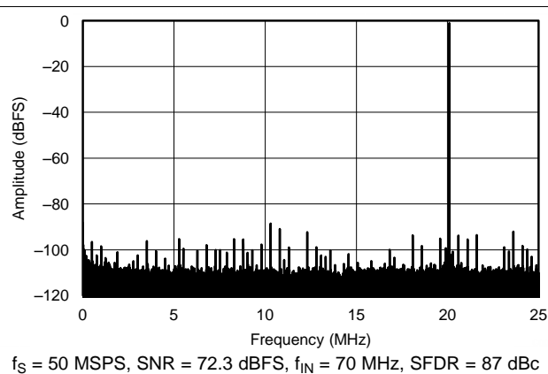
Figure 103. FFT for 70-MHz Input Signal, Dither Off
