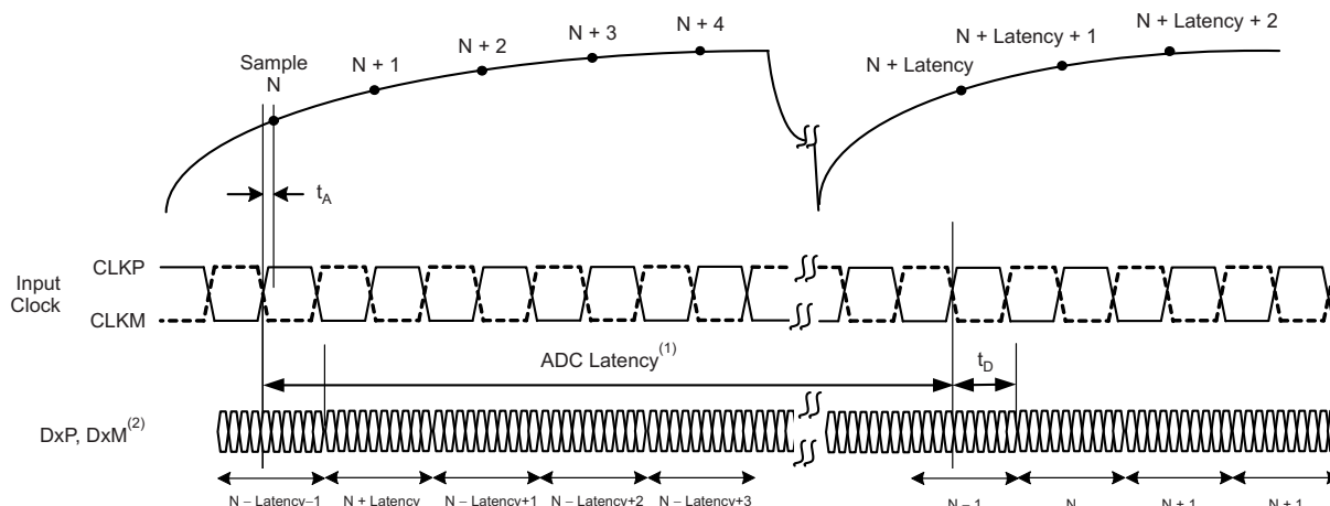
Figure 143. ADC Latency
