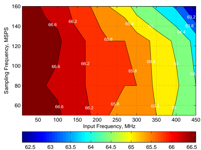
Figure 141. Signal-to-Noise Ratio (SNR) for 0-dB Gain
