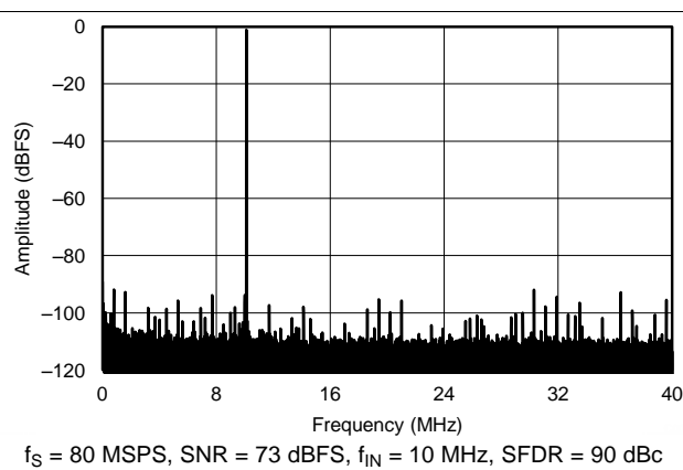
Figure 68. FFT for 10-MHz Input Signal, Dither Off
