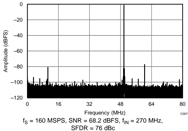
Figure 7. FFT for 270-MHz Input Signal, Dither On
