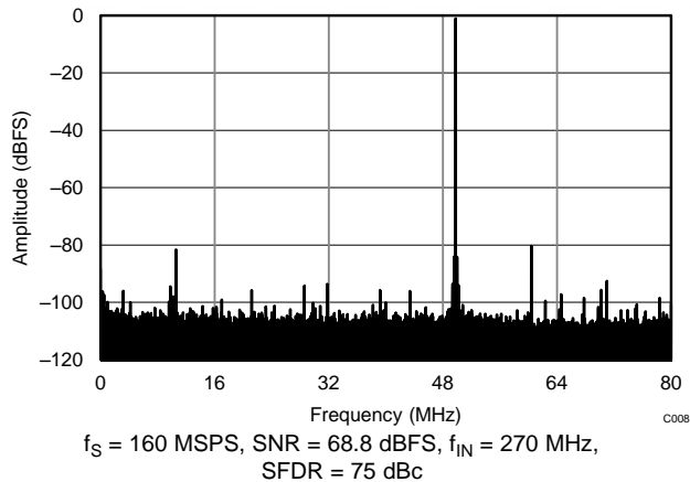
Figure 8. FFT for 270-MHz Input Signal, Dither Off
