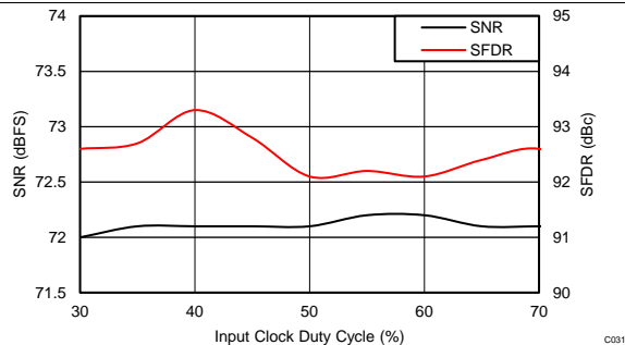
Figure 31. Performance vs Clock Duty Cycle (40 MHz)
