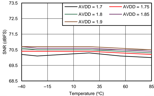
Figure 92. SNR vs AVDD Supply and Temperature
