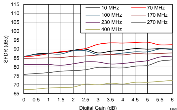
Figure 20. SFDR vs Digital Gain and Input Frequency
