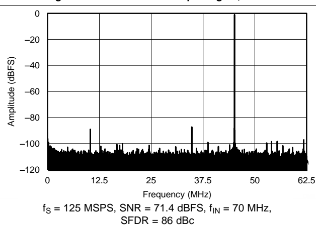
Figure 39. FFT for 170-MHz Input Signal, Dither Off
