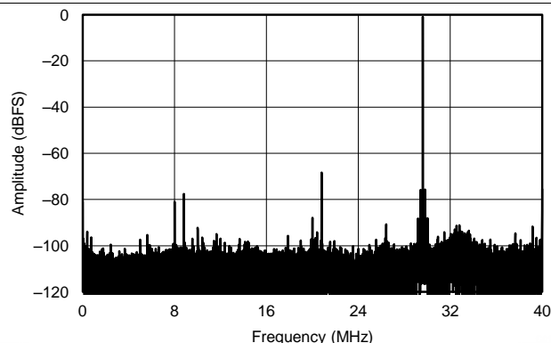
Figure 74. FFT for 270-MHz Input Signal, Dither Off
