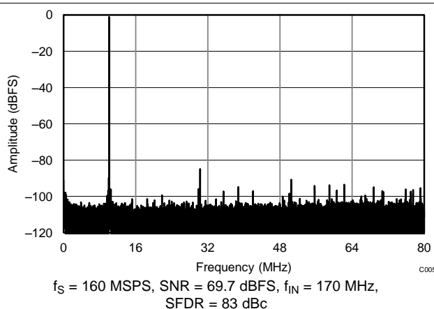
Figure 205. Performance FFT at 170 MHz (Mid Input Frequency)
