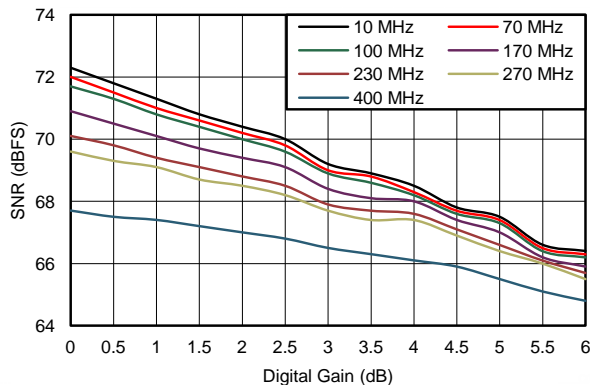
Figure 85. SNR vs Digital Gain and Input Frequency
