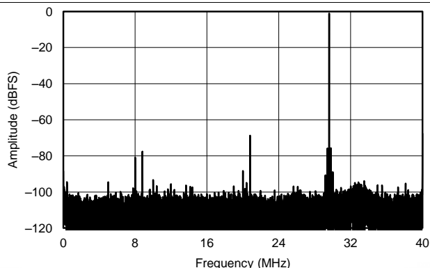
Figure 73. FFT for 270-MHz Input Signal, Dither On
