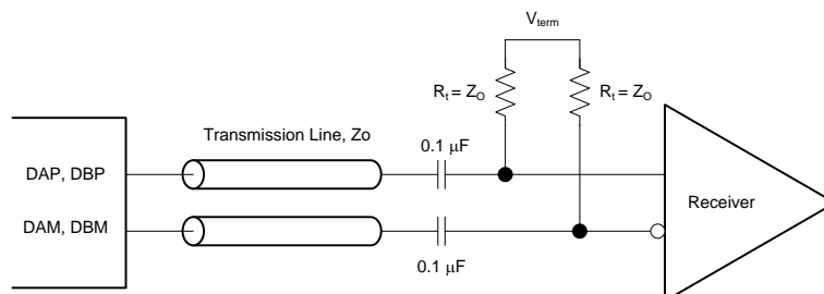
Figure 159. CML Output Connections
