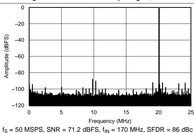
Figure 105. FFT for 170-MHz Input Signal, Dither Off
