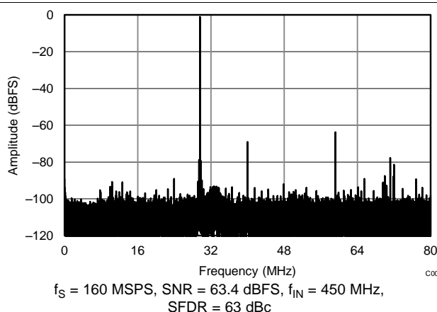
Figure 207. Performance FFT at 450 MHz (High Input Frequency)
