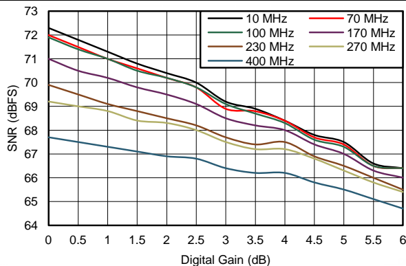
Figure 118. SNR vs Digital Gain and Input Frequency
