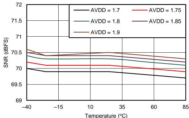
Figure 59. SNR vs AVDD Supply and Temperature
