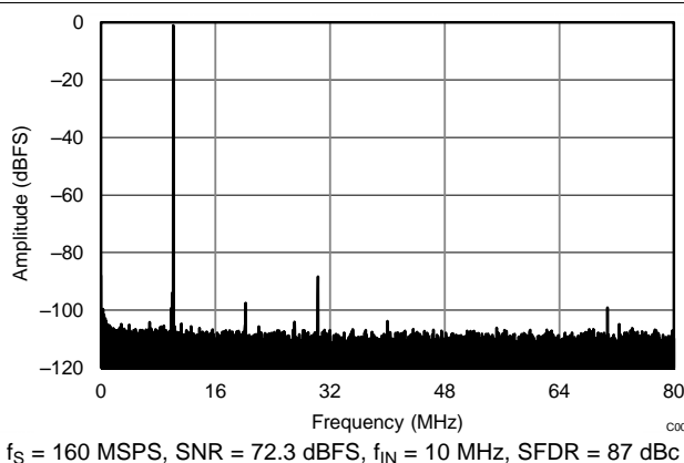
Figure 203. Performance FFT at 10 MHz (Low Input Frequency)
