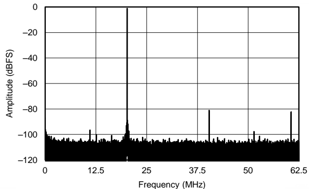
Figure 40. FFT for 270-MHz Input Signal, Dither On
