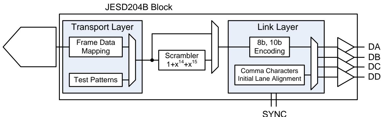
Figure 157. JESD204B Block
