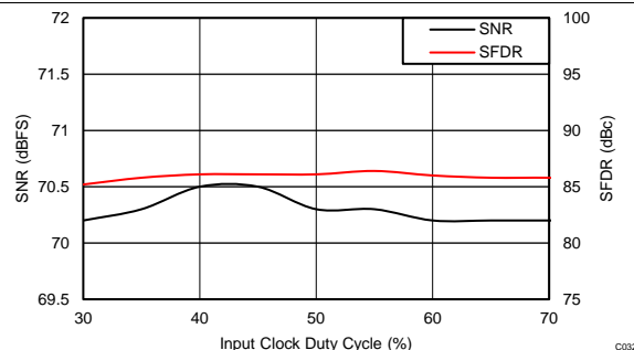
Figure 98. Performance vs Clock Duty Cycle (150 MHz)
