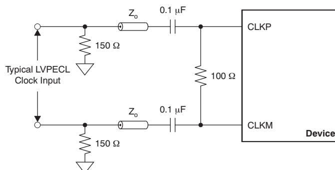
Figure 150. LVPECL Clock Driving Circuit
