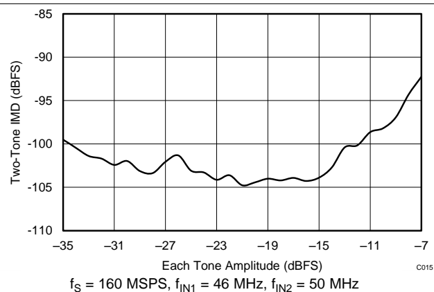
Figure 15. IMD vs Input Amplitude (46 MHz and 50 MHz)
