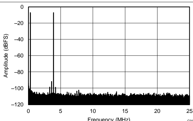
Figure 108. FFT for 450-MHz Input Signal, Dither On
