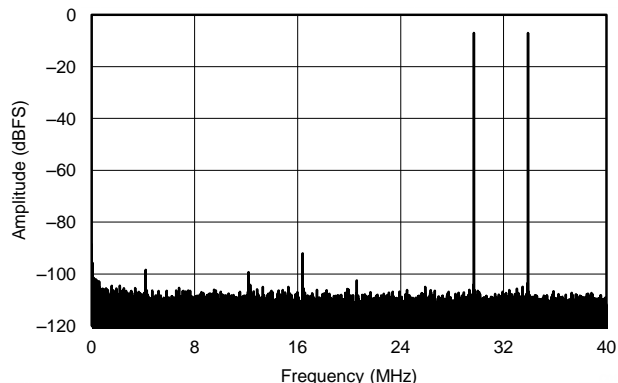
Figure 79. FFT for Two-Tone Input Signal ( -7\text{ dBFS} at 185 MHz and 190 MHz)
