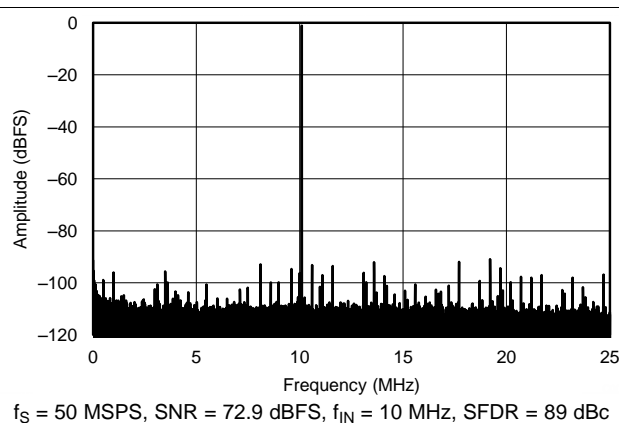
Figure 101. FFT for 10-MHz Input Signal, Dither Off
