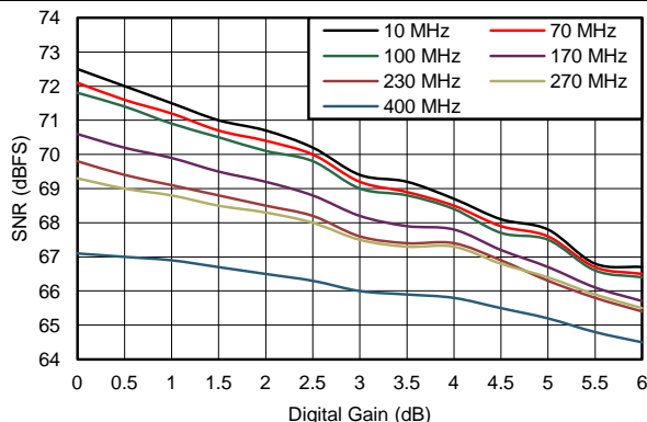
Figure 52. SNR vs Digital Gain and Input Frequency
