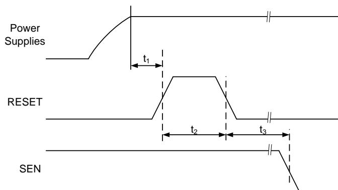
Figure 164. Initialization of Serial Registers after Power-Up
