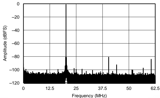
Figure 41. FFT for 270-MHz Input Signal, Dither Off
