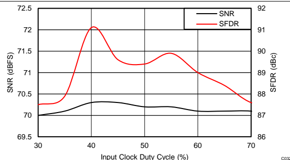
Figure 32. Performance vs Clock Duty Cycle (150 MHz)
