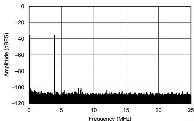
Figure 109. FFT for 450-MHz Input Signal, Dither Off
