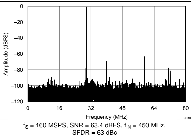
Figure 10. FFT for 450-MHz Input Signal, Dither Off
