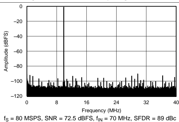
Figure 70. FFT for 70-MHz Input Signal, Dither Off
