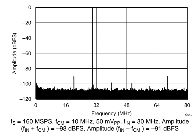
Figure 133. CMRR FFT
