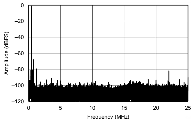
Figure 107. FFT for 270-MHz Input Signal, Dither Off
