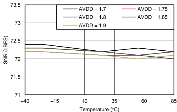
Figure 125. SNR vs AVDD Supply and Temperature
