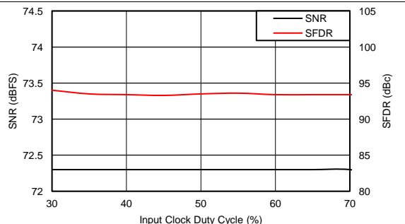
Figure 64. Performance vs Clock Duty Cycle (40 MHz)
