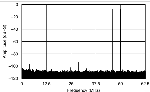
Figure 42. FFT for 450-MHz Input Signal, Dither On
