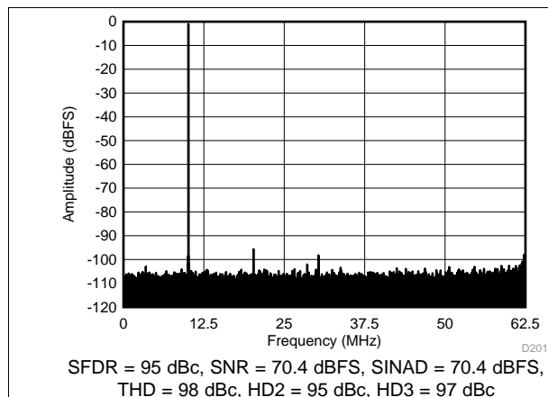
Figure 141. FFT for 10-MHz Input Signal (Chopper On, Dither On)
