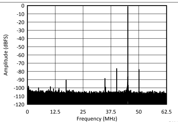
Figure 122. Power-Supply Rejection Ratio Spectrum
