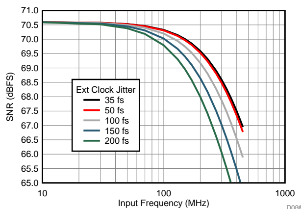
Figure 137. SNR vs Frequency for Different Clock Jitter
