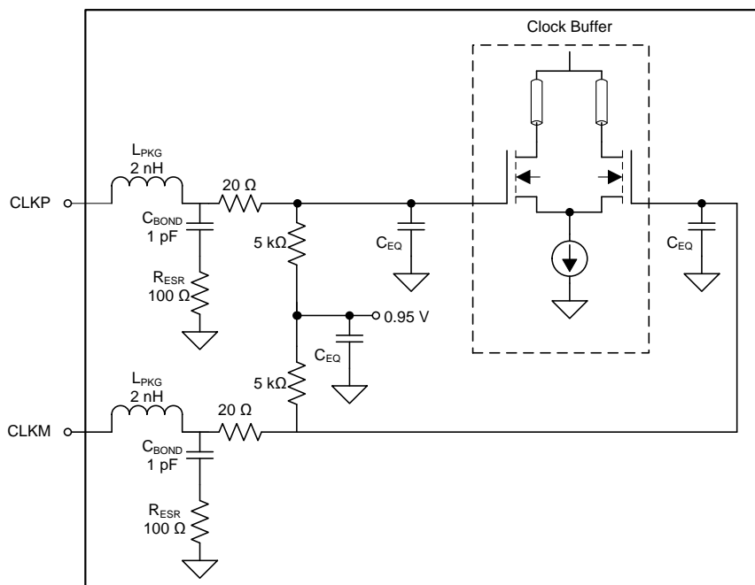
Figure 135. Internal Clock Buffer
