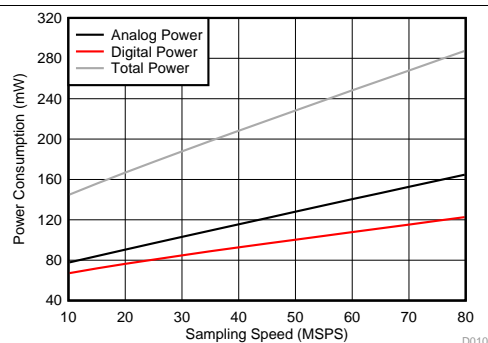
Figure 126. Power vs Sampling Frequency (One-Wire Mode)
