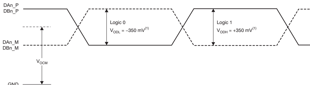
Figure 129. Serial LVDS Output Voltage Levels
