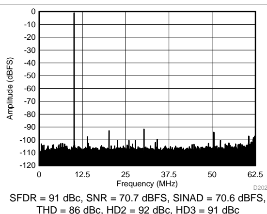
Figure 142. FFT for 10-MHz Input Signal (Chopper On, Dither Off)
