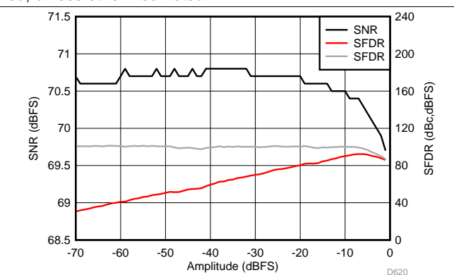
Figure 50. Performance vs Input Amplitude (170 MHz)
