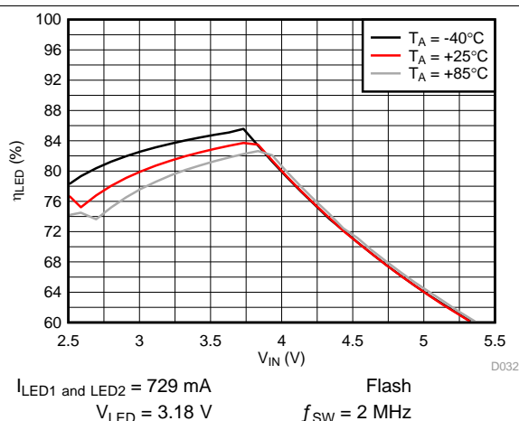
Figure 43. LED Efficiency vs Input Voltage
