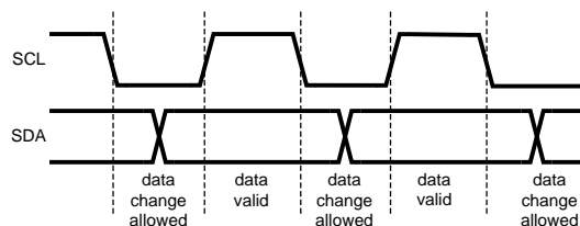
Figure 32. Data Validity Data
