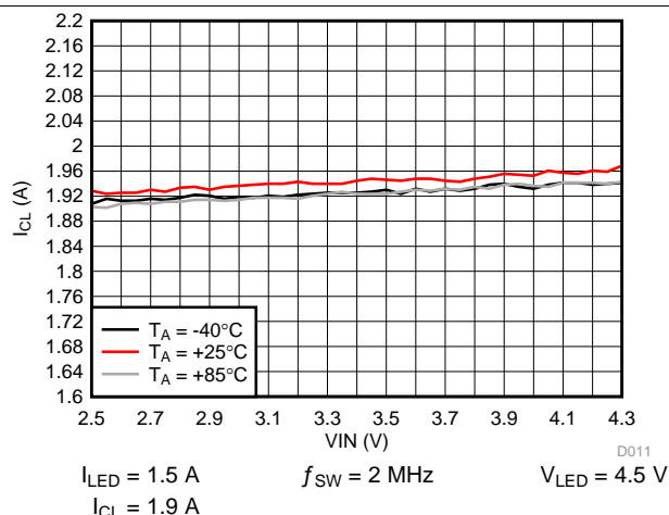
Figure 21. Inductor Current Limit vs Input Voltage
