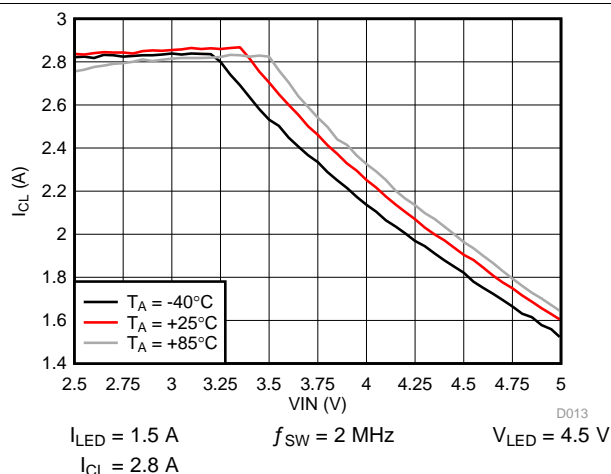
Figure 23. Inductor Current Limit vs Input Voltage
