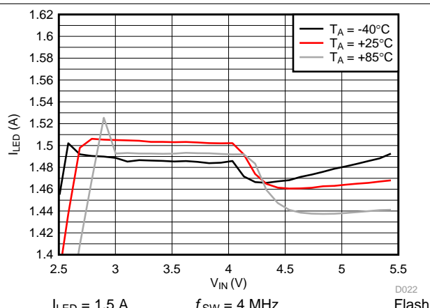
Figure 9. LED2 Current vs Input Voltage
