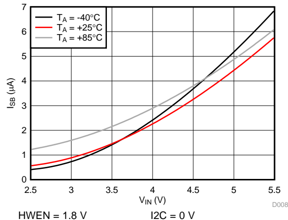
Figure 19. Standby Current vs Input Voltage
