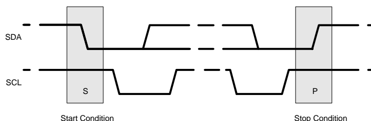
Figure 33. Start and Stop Conditions
