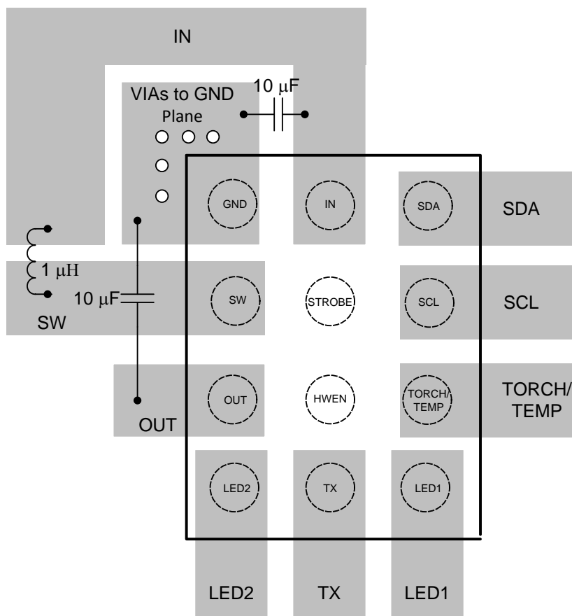
Figure 56. Layout Example
