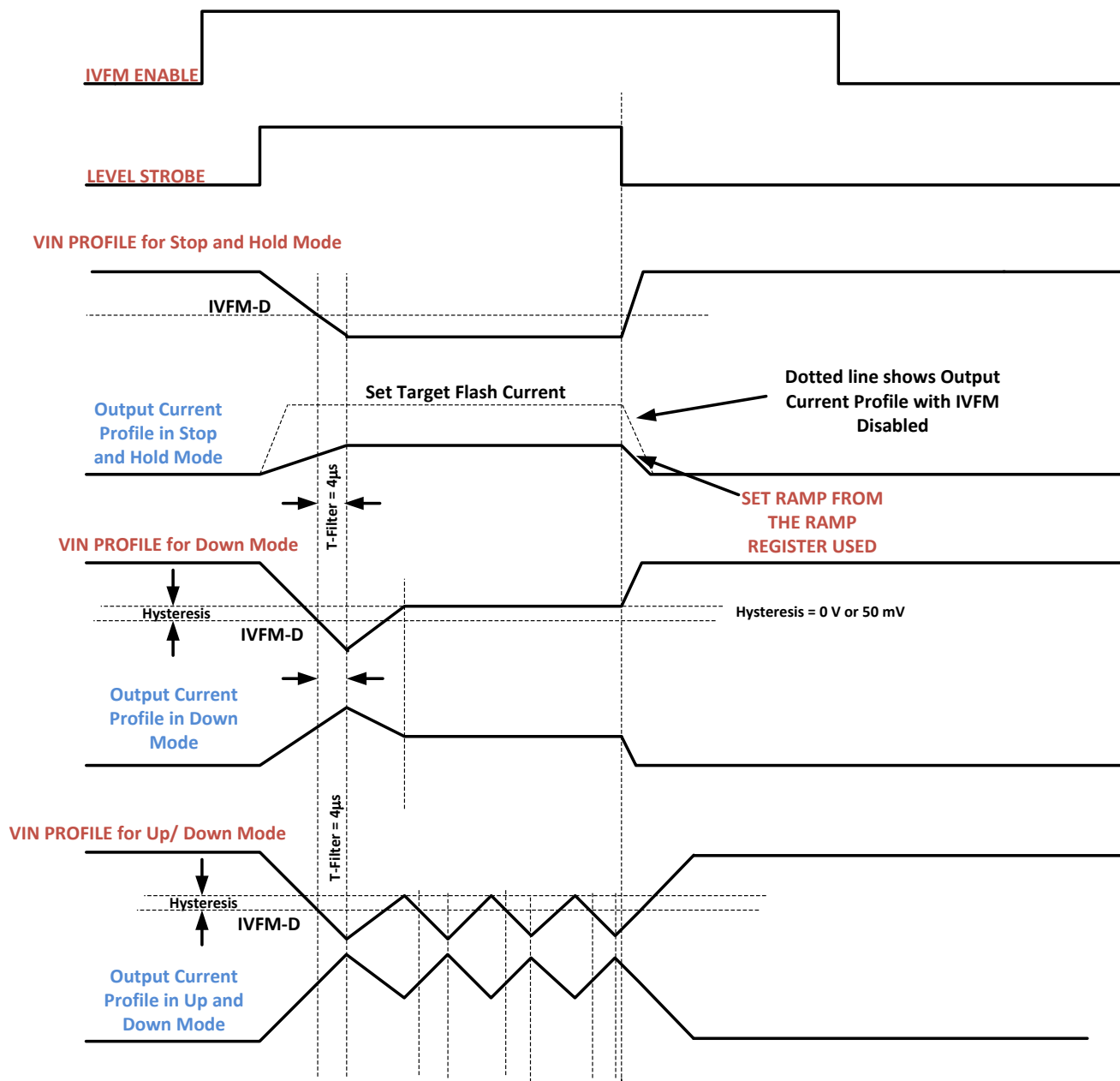
Figure 30. IVFM Modes
