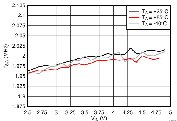
Figure 25. 2-MHz Switching Frequency vs Input Voltage
