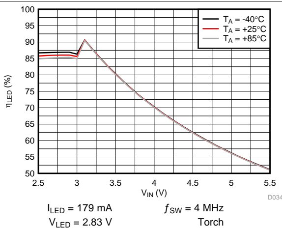
Figure 45. LED Efficiency vs Input Voltage
