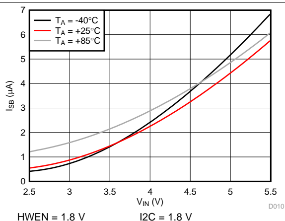
Figure 18. Standby Current vs Input Voltage
