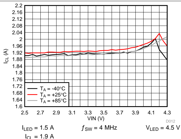
Figure 22. Inductor Current Limit vs Input Voltage
