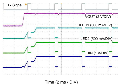
Figure 48. Start-Up
