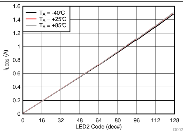
Figure 3. LED2 Flash Current vs Brightness Code
