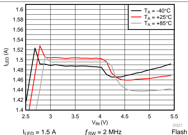
Figure 8. LED2 Current vs Input Voltage
