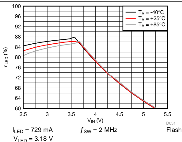
Figure 42. LED Efficiency vs Input Voltage
