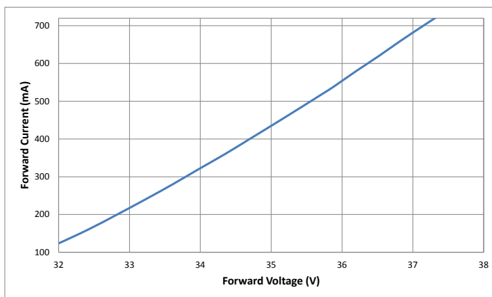
Forward Current vs. Forward Voltage @ 85°C
