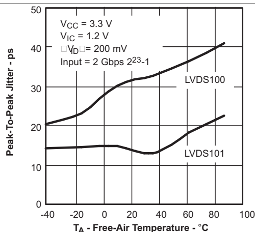
Figure 20. SN65LVDS100 Peak-to-Peak Jitter vs Free-Air Temperature
