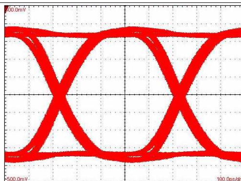
Horizontal Scale= 100 ps/div LVPECL-to-LVDS Figure 26. SN65LVDS100 Gbps, 2^{23} - 1 PRBS
