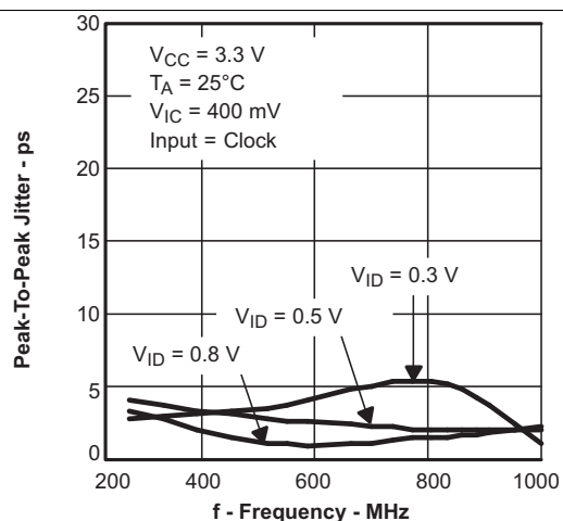
Figure 8. SN65LVDS100 Peak-to-Peak Jitter vs Frequency
