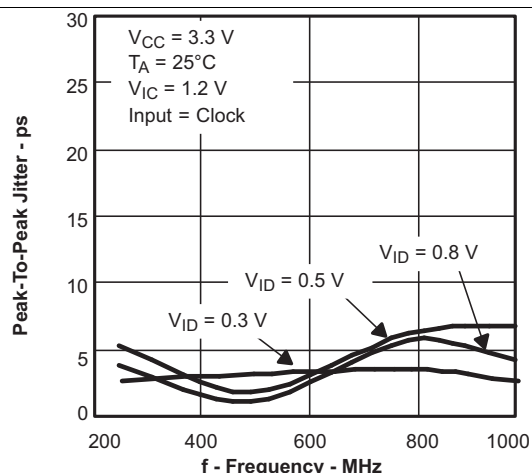
Figure 12. SN65LVDS100 Peak-to-Peak Jitter vs Frequency
