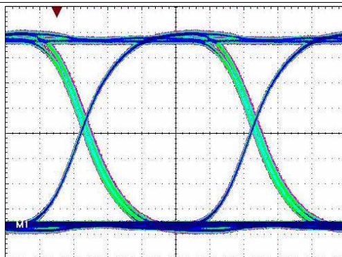
Horizontal Scale= 100 ps/div LVDS-to-LVPECL Figure 28. SN65LVDS101 Gbps, 2^{23} - 1 PRBS
