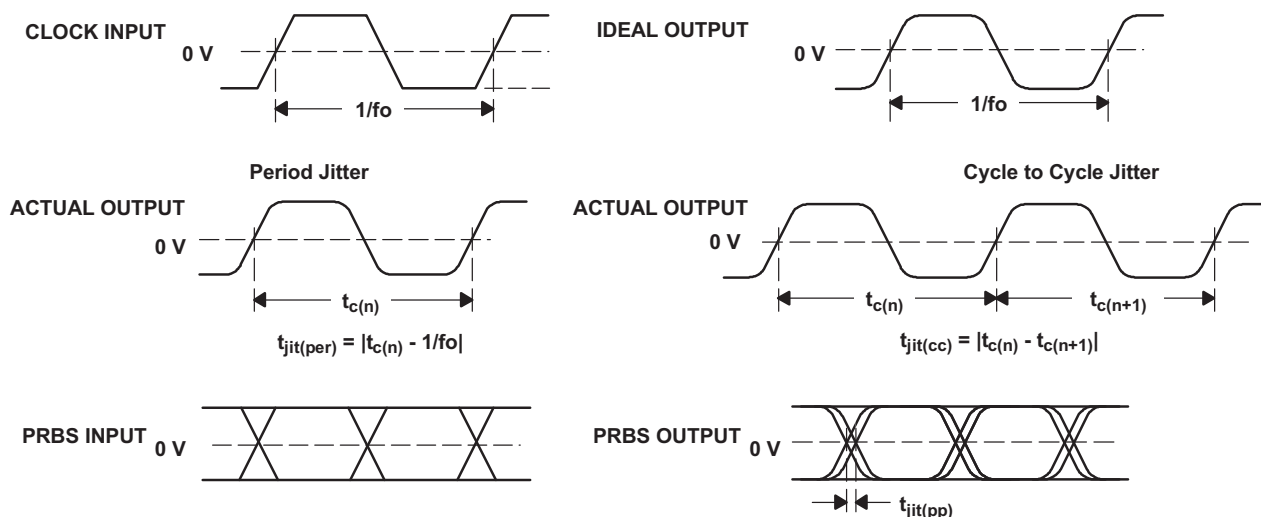
Figure 34. Driver Jitter Measurement Waveforms
