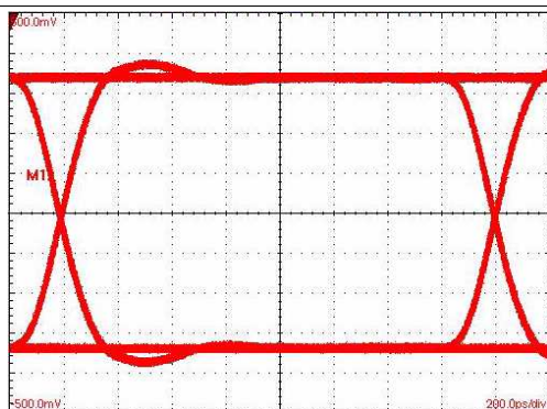
Horizontal Scale= 200 ps/div LVPECL-to-LVDS Figure 25. SN65LVDS100 Mbps, 2^{23} - 1 PRBS
