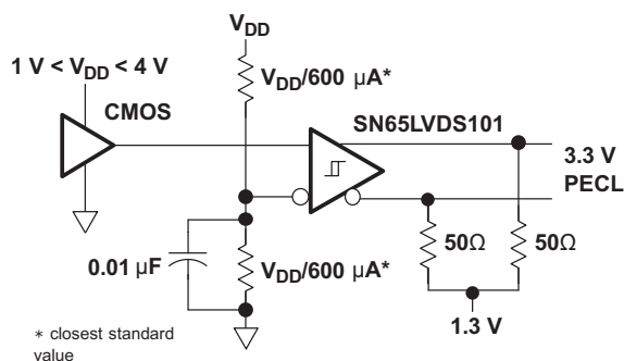
Figure 49. Single-Ended CMOS to 3.3-V PECL Translation
