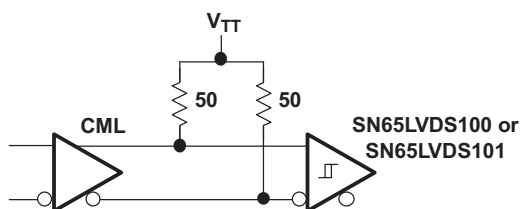
Figure 46. CML to LVDS or 3.3-V PECL Translation
