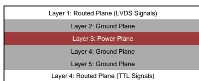
Figure 54. Six-Layer PCB Board
