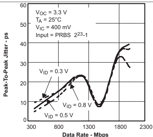
Figure 9. SN65LVDS100 Peak-to-Peak Jitter vs Data Rate
