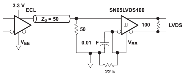
Figure 47. Single-Ended 3.3-V PECL to LVDS Translation
