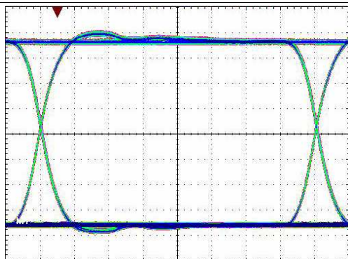
Horizontal Scale= 200 ps/div LVDS-to-LVPECL Figure 27. SN65LVDS101 Mbps, 2^{23} - 1 PRBS
