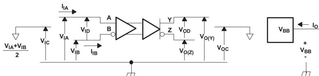
Figure 30. Voltage and Current Definitions
