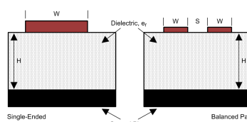
Figure 51. Microstrip Topology
