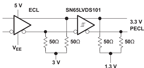
Figure 45. 5-V PECL to 3.3-V PECL Translation
