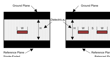
Figure 52. Stripline Topology
