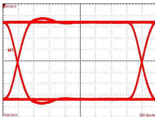
Figure 42. SN65LVDS100 Mbps, 2^{23} - 1 PRBS
