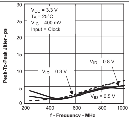
Figure 10. SN65LVDS101 Peak-to-Peak Jitter vs Frequency
