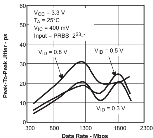
Figure 11. SN65LVDS101 Peak-to-Peak Jitter vs Data Rate
