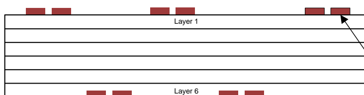
Figure 56. Staggered Trace Layout
