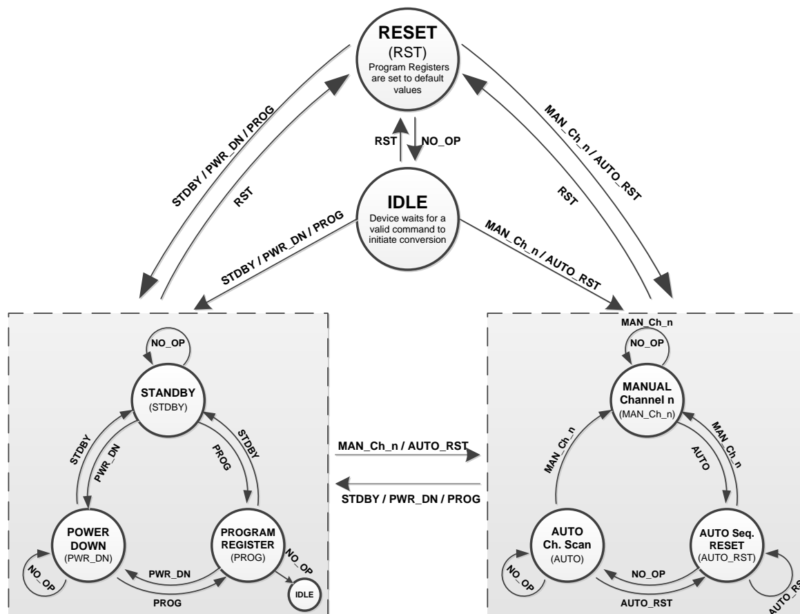
Figure 76. State Transition Diagram
