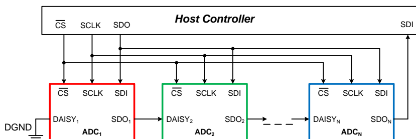
Figure 73. Daisy-Chain Connection Schematic
