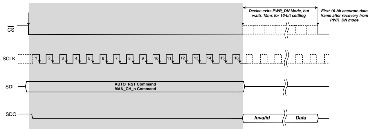
Figure 80. Exit PWR_DN Mode Timing Diagram
