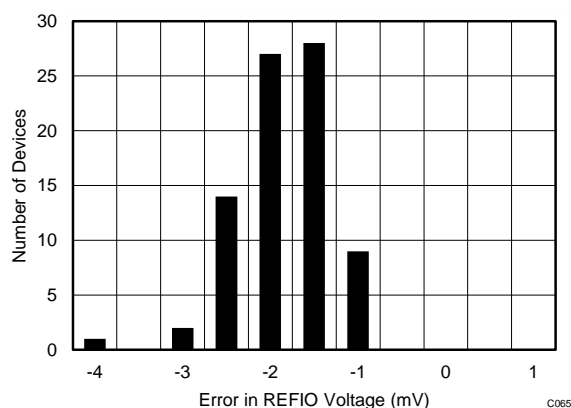
Figure 59. Solder Heat Shift Distribution Histogram
