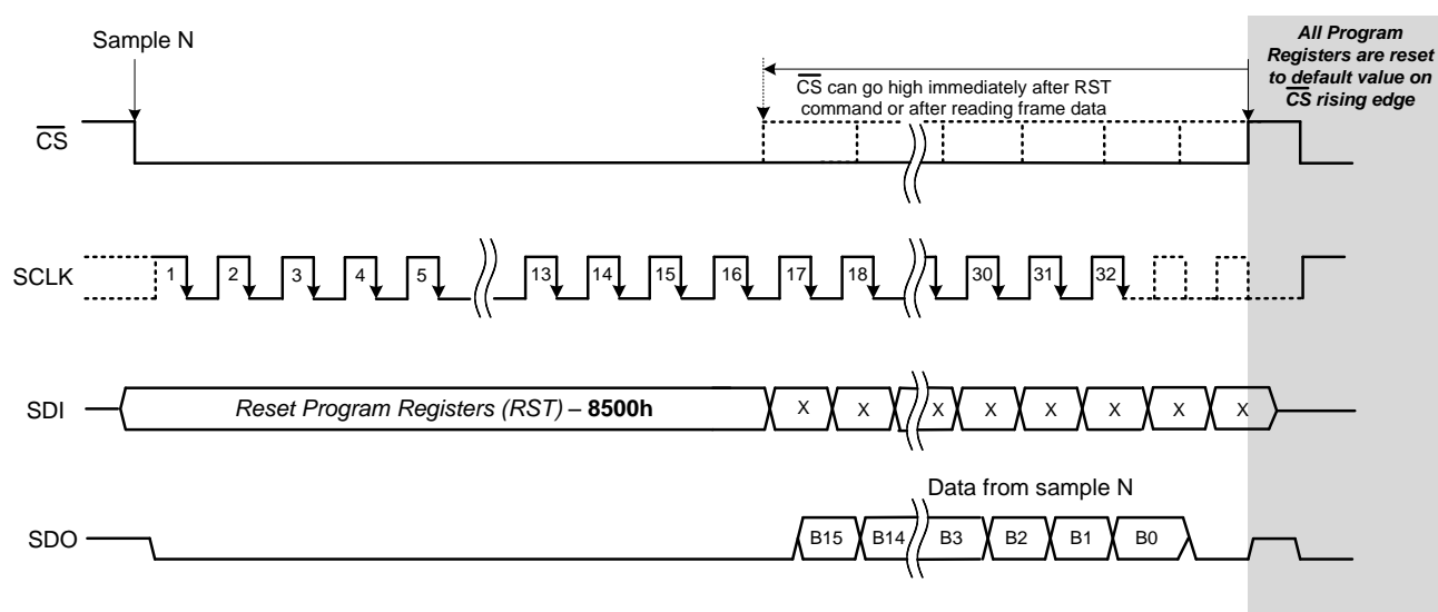
Figure 87. Reset Program Registers (RST) Timing Diagram
