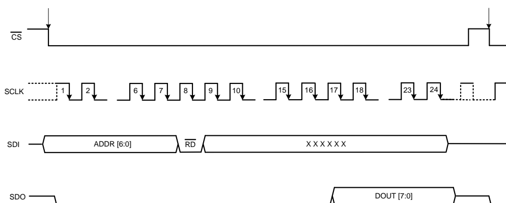
Figure 89. Program Register Read Cycle Timing Diagram
