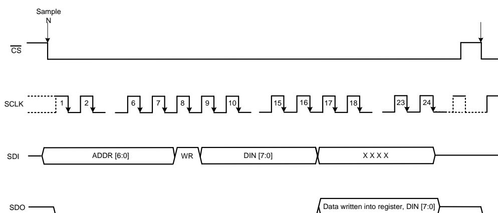
Figure 88. Program Register Write Cycle Timing Diagram
