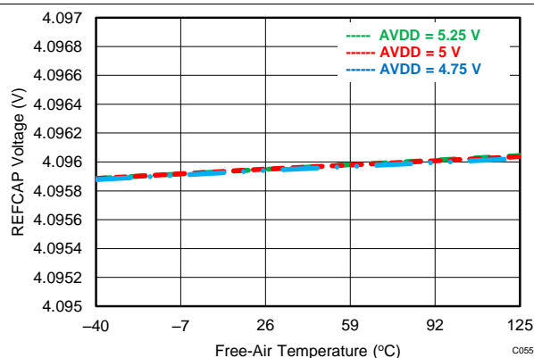
Figure 63. Variation of the Reference Buffer Output (REFCAP) Across Supply and Temperature
