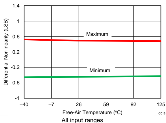
Figure 12. DNL vs Temperature
