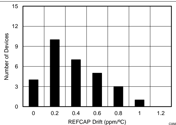
Figure 64. Reference Buffer Temperature Drift Histogram
