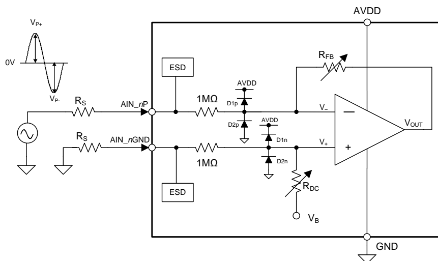
Figure 52. Input Overvoltage Protection Circuit Schematic
