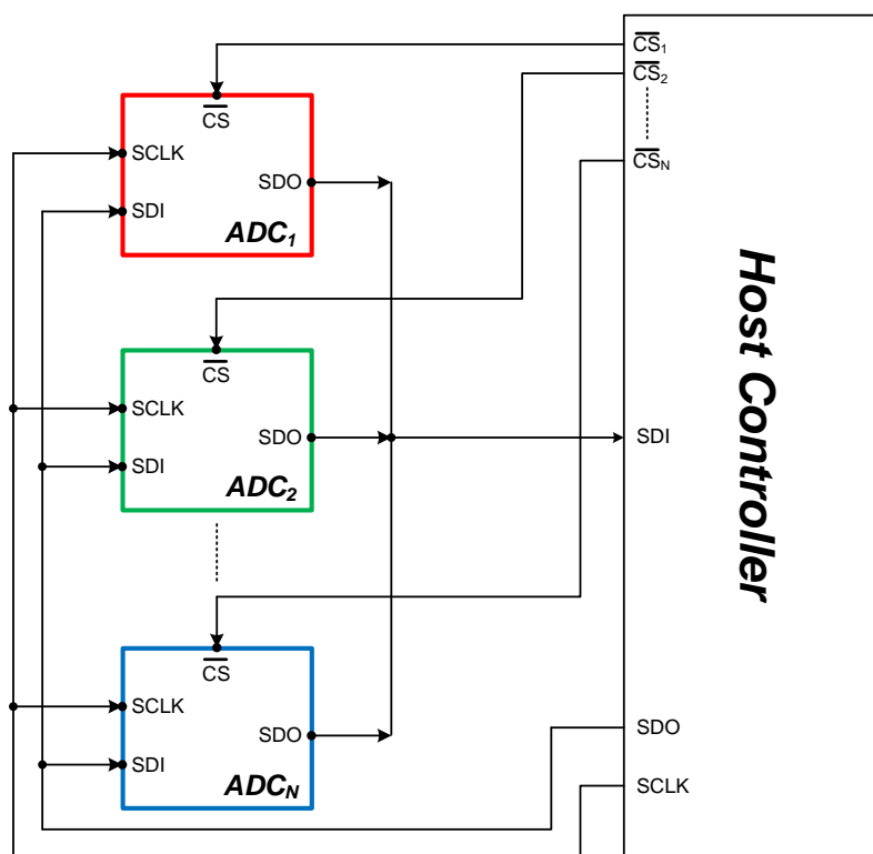
Figure 75. Star Topology Connection Schematic
