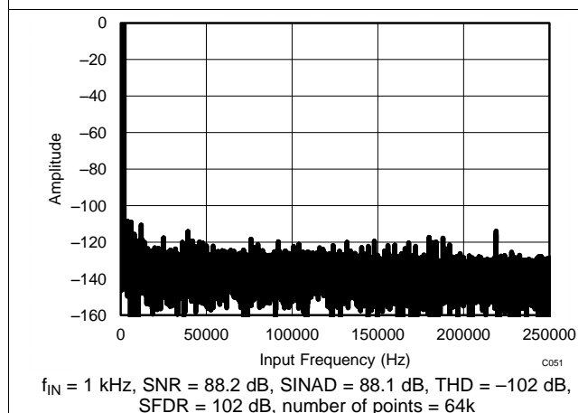
Figure 67. Typical FFT Plot (AUX Channel)
