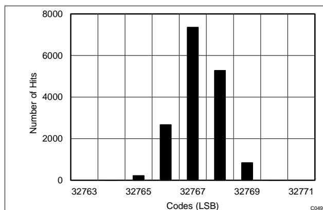
Figure 65. DC Histogram for Mid-Scale Input (AUX Channel)
