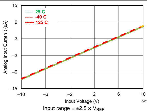
Figure 3. Input Current vs Temperature
