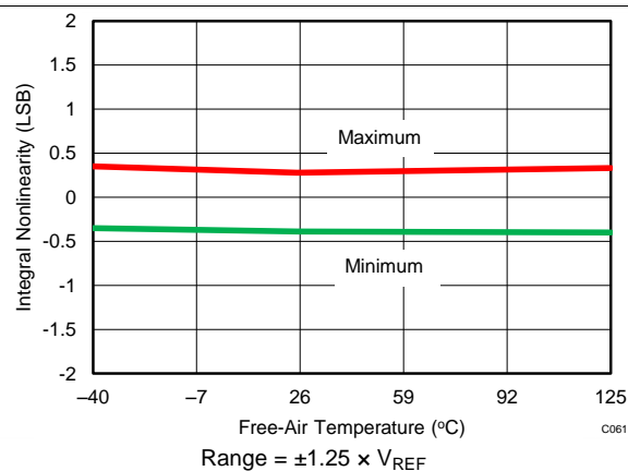
Figure 19. INL vs Temperature ( \pm 1.25 \times V_{REF} )
