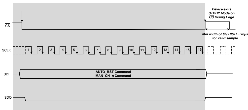
Figure 78. Exit STDBY Mode Timing Diagram
