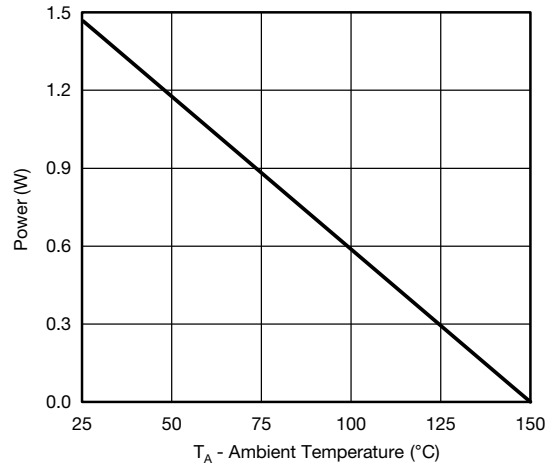
Power Derating
