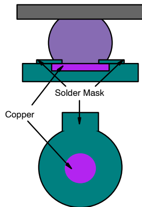
FIGURE 3. SMD
