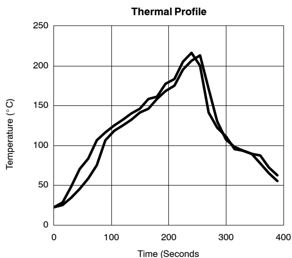
FIGURE 6. Reflow Profile
