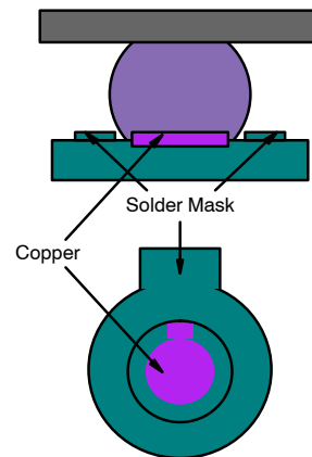
FIGURE 4. NSMD
