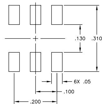
SUGGESTED LAND PATTERN
