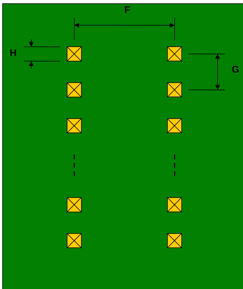
Bottom View (DIP Pins)
