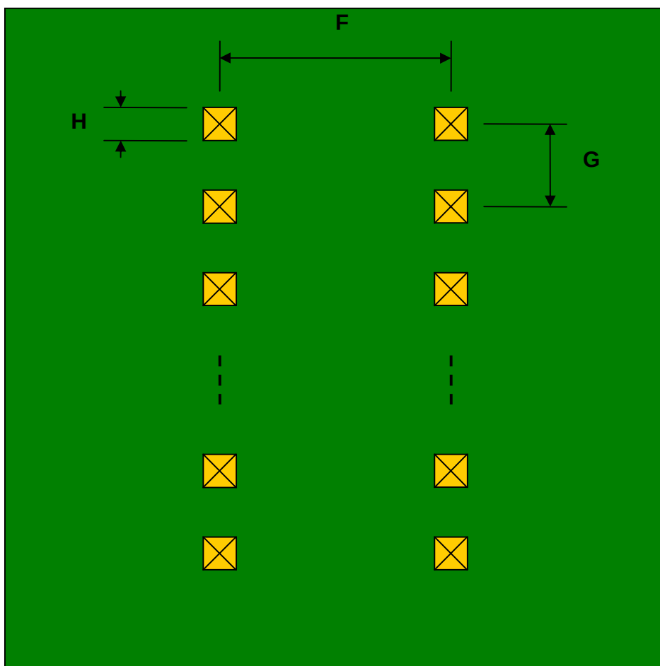
Bottom View (DIP Pins)
