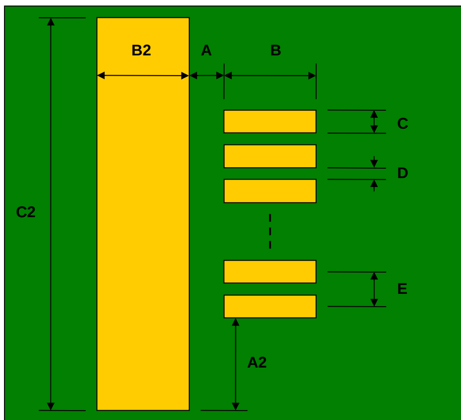
Top View (SMT Footprint)
