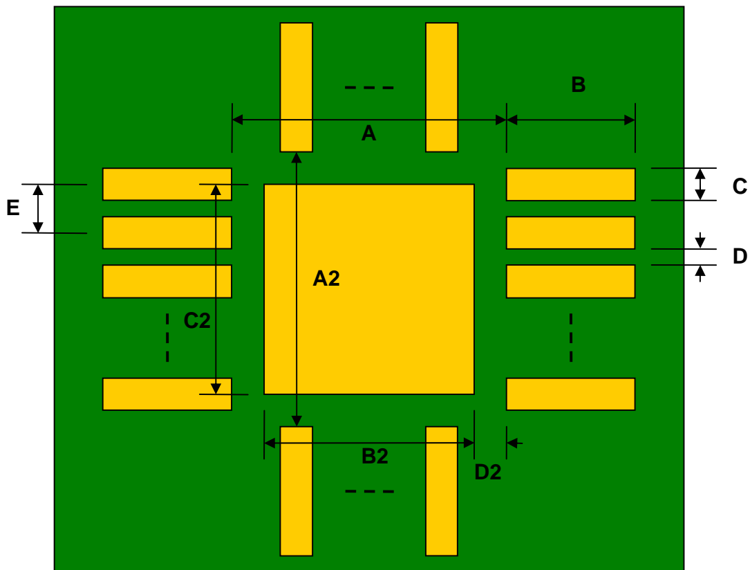
Top View (SMT Footprint)
