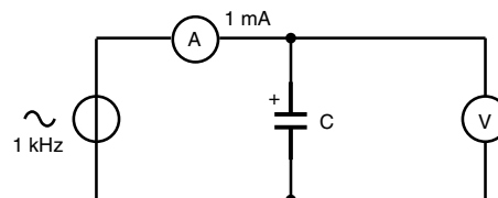
Fig. 15 - Test Circuit for R_I Measurement
