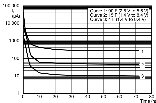
Fig. 17 - Typical Leakage Current at 20 °C as a Function of Time
