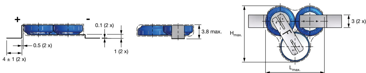
Fig. 8 - Form E3: Surface Mount Flat
