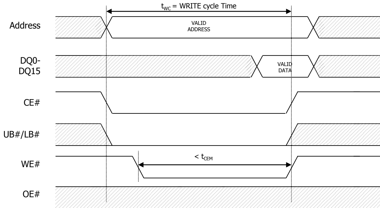
Figure 3. Asynchronous WRITE operation
