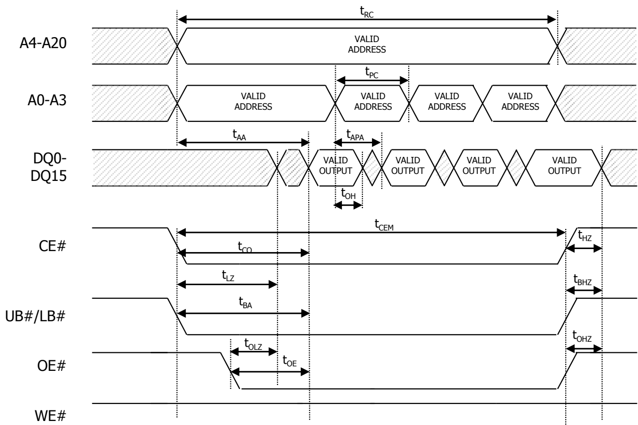
Figure 14: PAGE MODE READ
