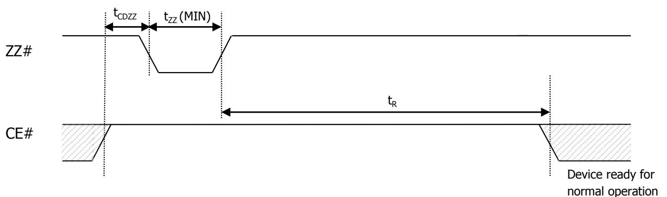
Figure 12: DPD Entry and Exit Timing
