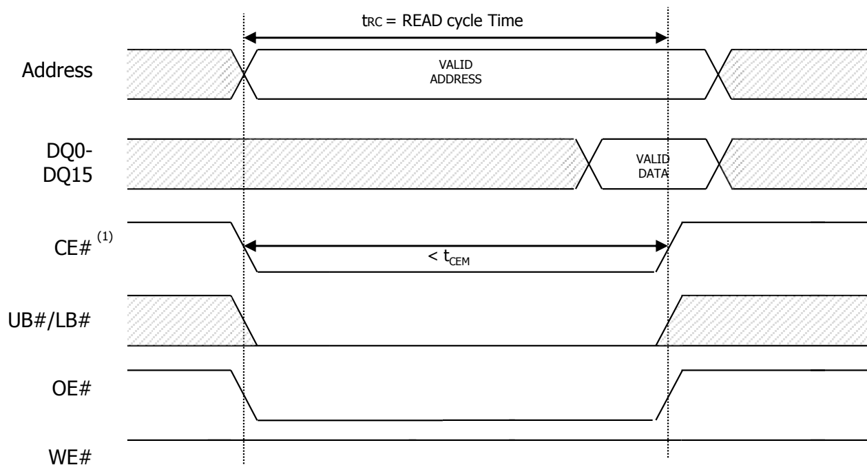
Figure 2. Asynchronous Read Operation
