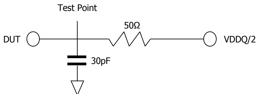
Figure 9. Output Load Circuit
