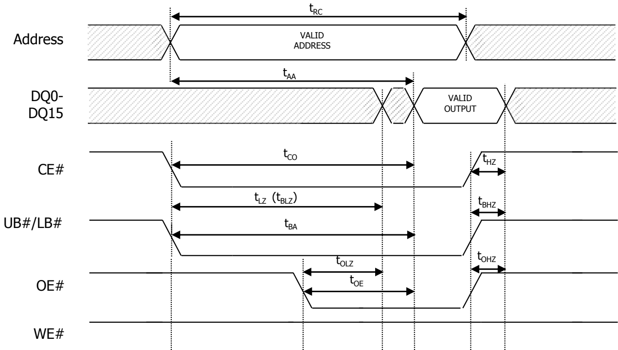
Figure 13: Single Read Operation
