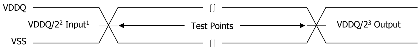
Figure 8. AC Input/Output Reference Waveform
