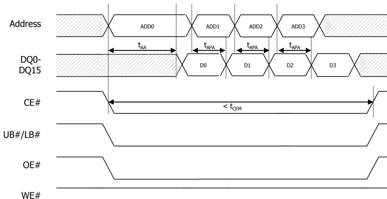
Figure 4. Page Mode READ Operation
