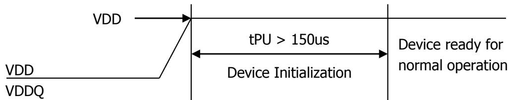
Figure 1: Power-Up Initialization Timing
