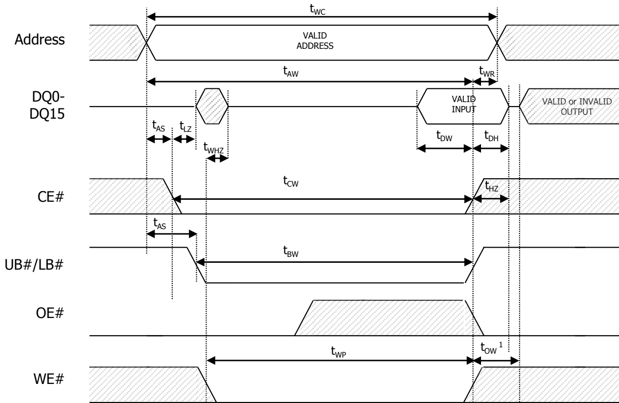
Figure 16: LB#/UB#-Controlled Asynchronous WRITE
