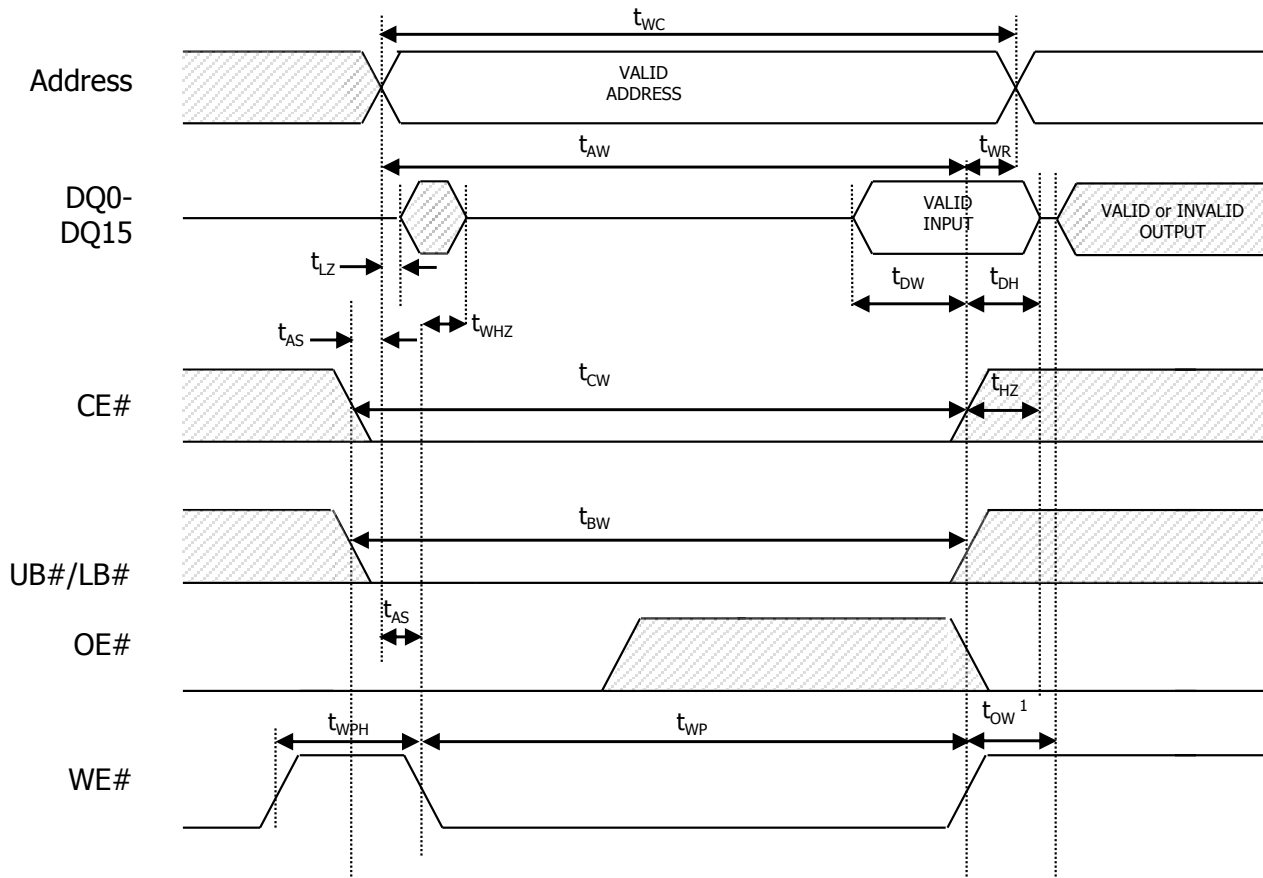
Figure 17: WE#-Controlled Asynchronous WRITE
