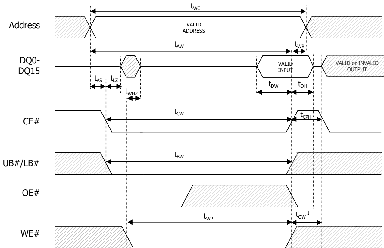
Figure 15: CE#-Controlled Asynchronous WRITE
