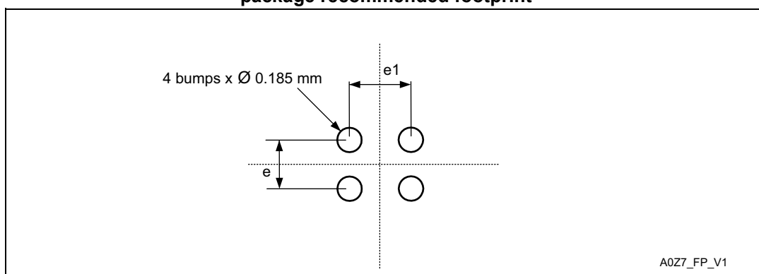
Figure 14. Thin WLCSP- 4-bump, 0.833 x 0.833 mm, wafer level chip scale package recommended footprint
