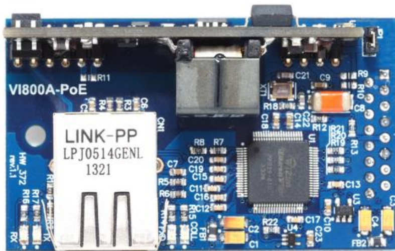
Figure 3-1 – VI800A-PoE module
