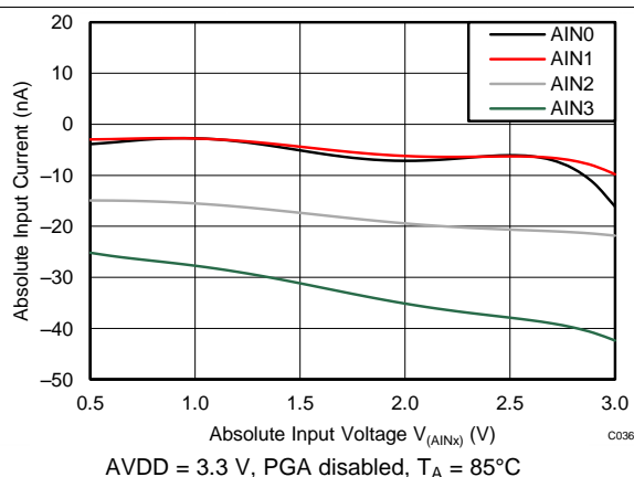
Figure 23. Absolute Input Current vs Absolute Input Voltage
