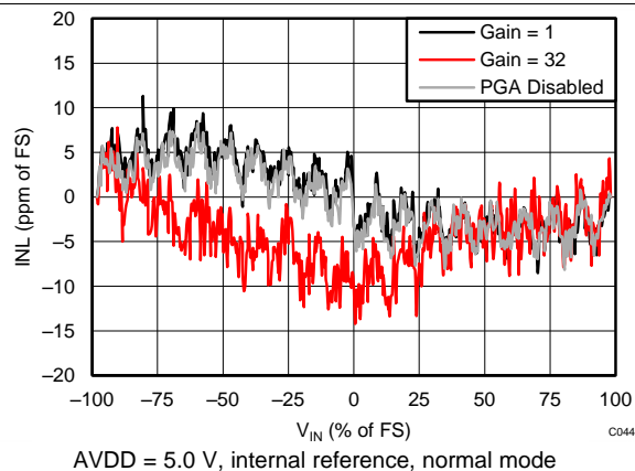
Figure 10. Integral Nonlinearity vs Differential Input Signal
