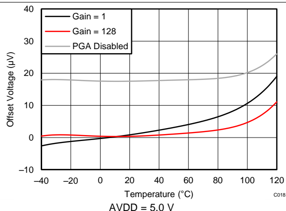
Figure 4. Input-Referred Offset Voltage vs Temperature
