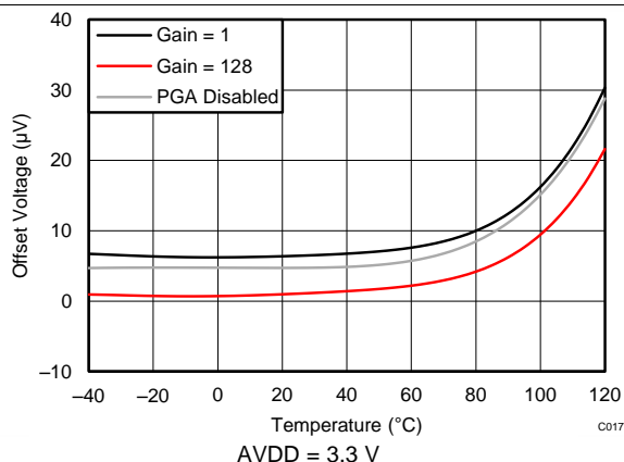
Figure 3. Input-Referred Offset Voltage vs Temperature
