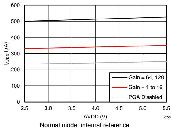
Figure 33. I_{AVDD} vs AVDD
