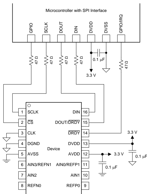
Figure 72. Serial Interface Connections
