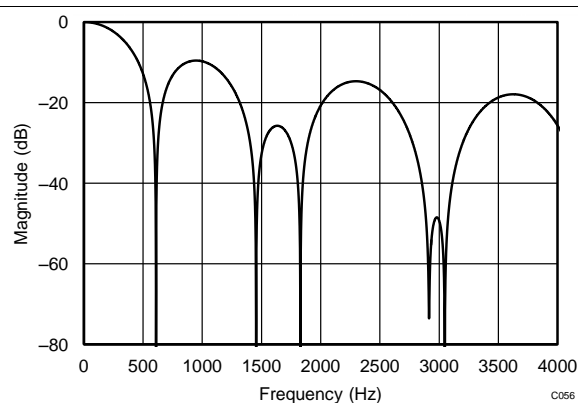
Figure 55. Filter Response (DR = 175 SPS)
