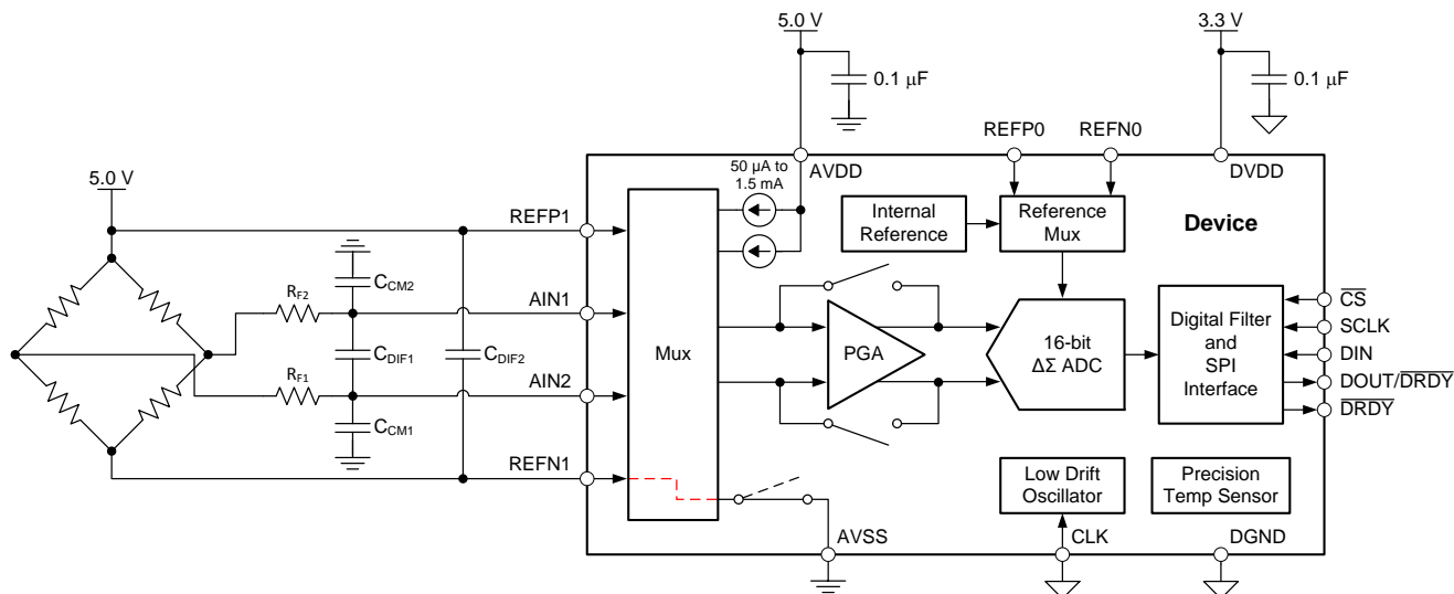
Figure 82. Bridge Measurement
