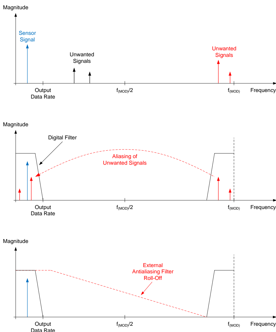
Figure 73. Effect of Aliasing
