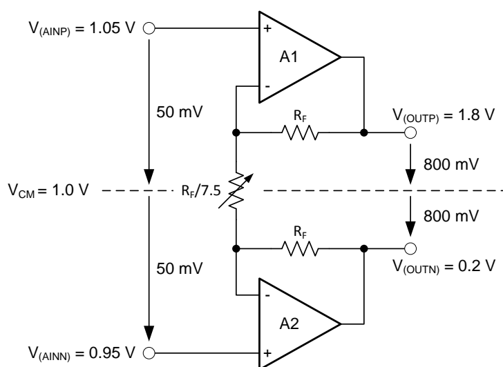
Figure 43. Example where V_{CM} is at Lowest Limit
