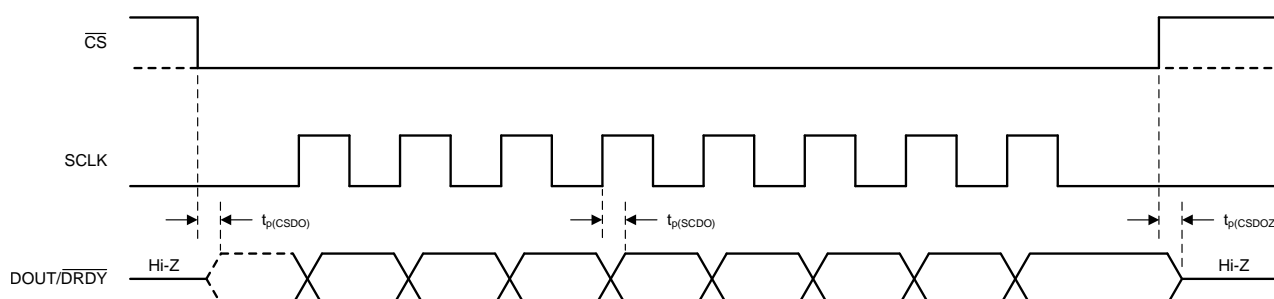
Figure 2. Serial Interface Switching Characteristics
