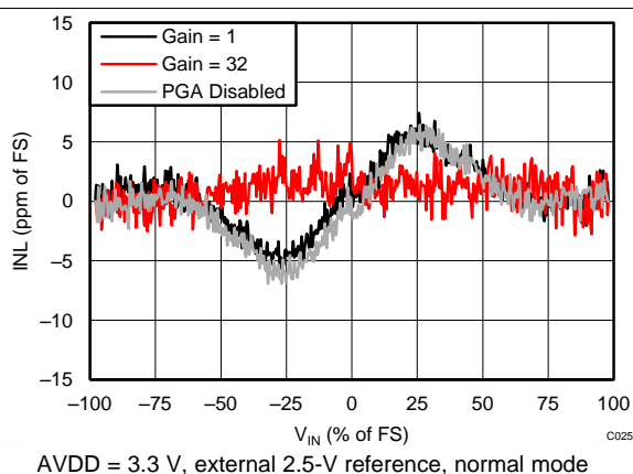
Figure 7. Integral Nonlinearity vs Differential Input Signal
