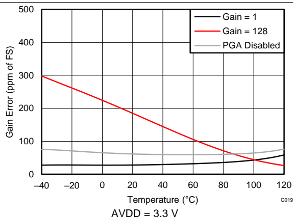
Figure 5. Gain Error vs Temperature
