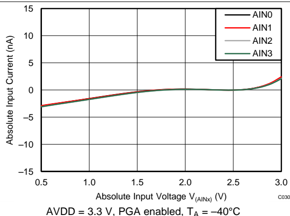
Figure 15. Absolute Input Current vs Absolute Input Voltage
