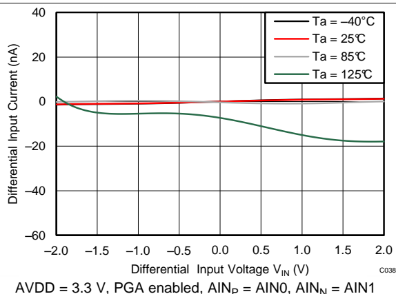
Figure 19. Differential Input Current vs Differential Input Voltage
