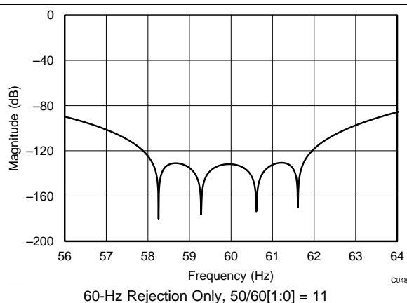
Figure 51. Detailed View of Filter Response (DR = 20 SPS)
