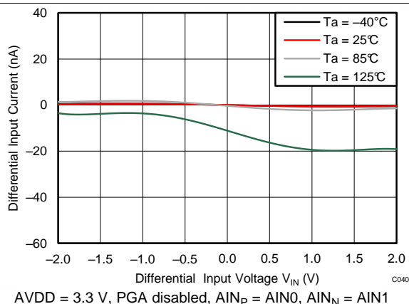
Figure 25. Differential Input Current vs Differential Input Voltage
