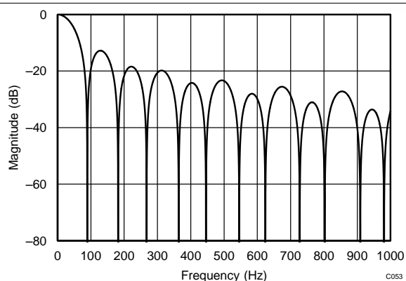
Figure 54. Filter Response (DR = 90 SPS)
