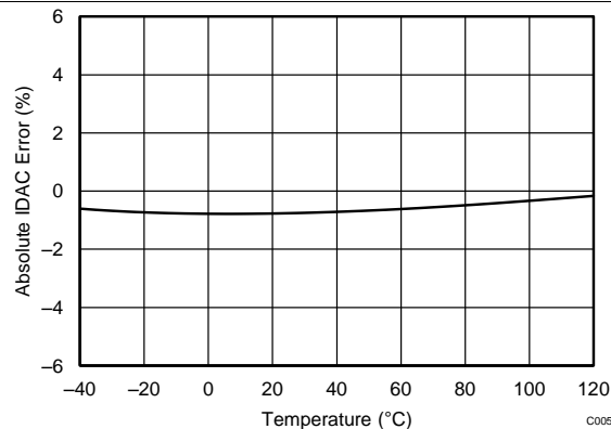
Figure 28. IDAC Accuracy vs Temperature
