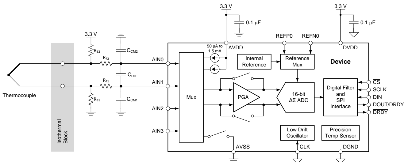
Figure 74. Thermocouple Measurement
