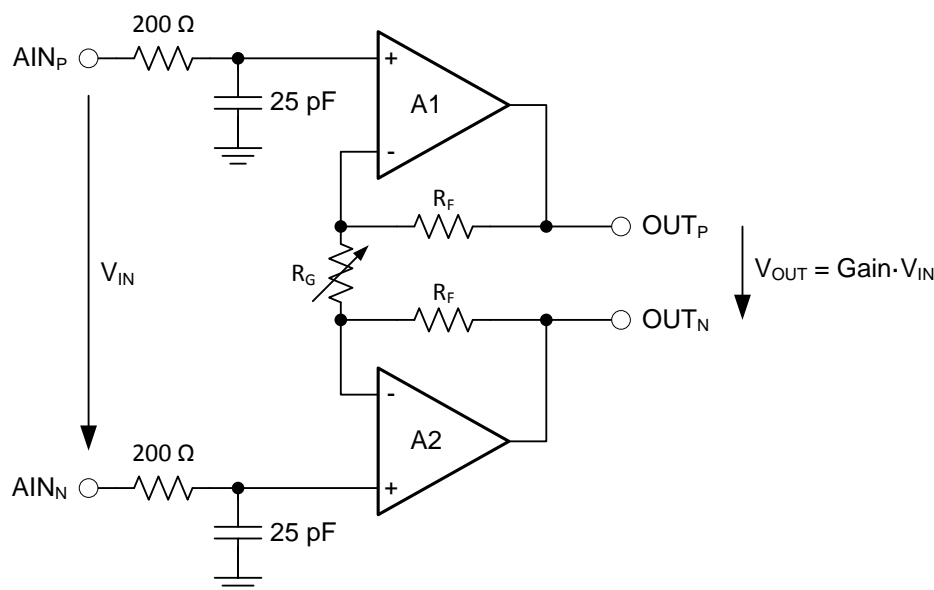
Figure 39. Simplified PGA Diagram
