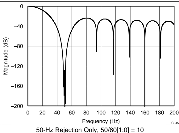
Figure 48. Filter Response (DR = 20 SPS)
