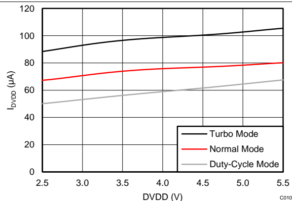
Figure 34. I_{DVDD} vs DVDD
