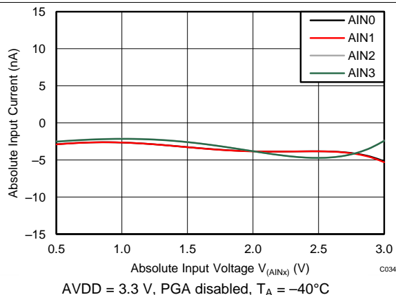
Figure 21. Absolute Input Current vs Absolute Input Voltage
