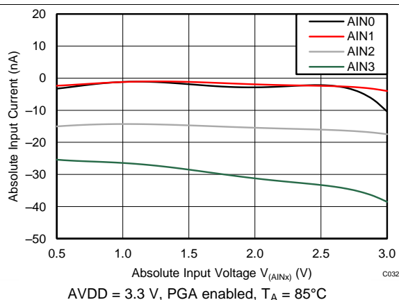
Figure 17. Absolute Input Current vs Absolute Input Voltage
