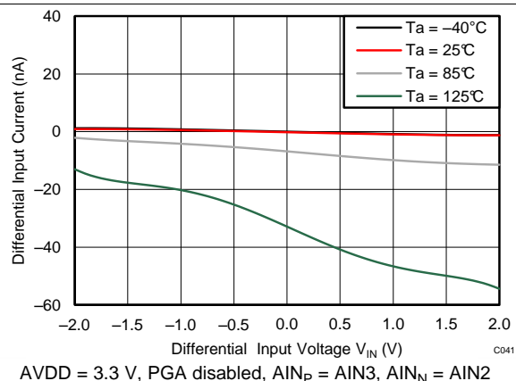
Figure 26. Differential Input Current vs Differential Input Voltage
