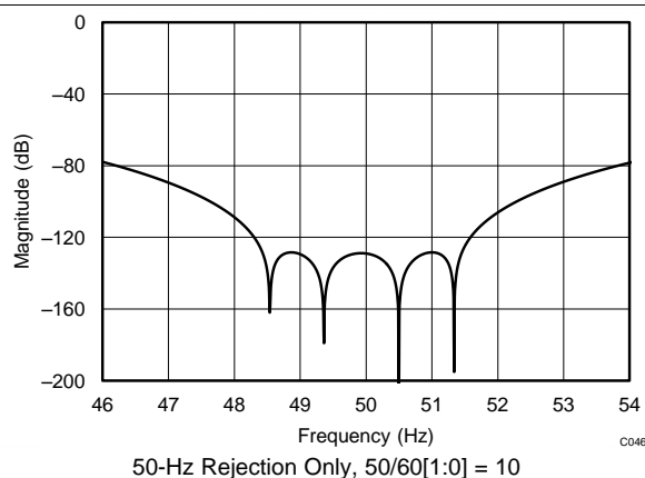
Figure 49. Detailed View of Filter Response (DR = 20 SPS)
