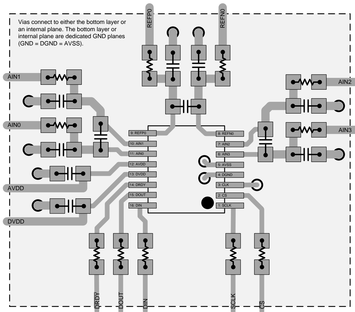
Figure 86. Layout Example
