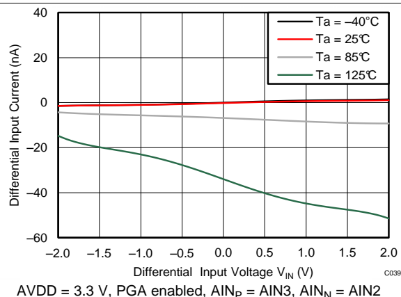
Figure 20. Differential Input Current vs Differential Input Voltage
