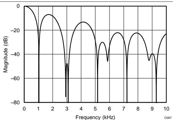
Figure 56. Filter Response (DR = 330 SPS)
