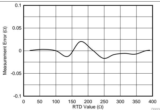
Figure 80. Resistance Measurement Error vs R_{RTD}
