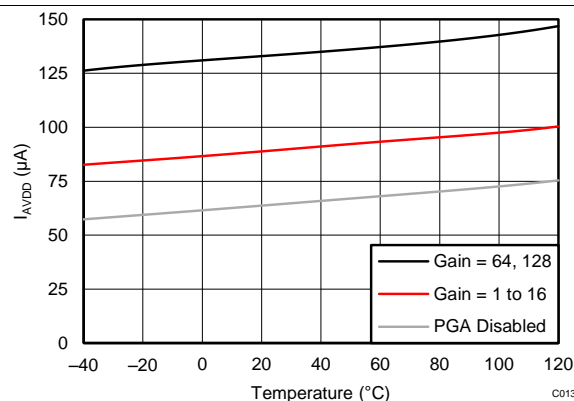
Figure 30. I_{AVDD} vs Temperature
