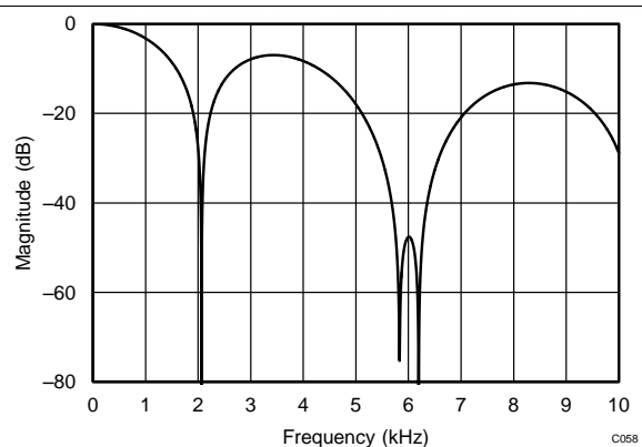
Figure 57. Filter Response (DR = 600 SPS)
