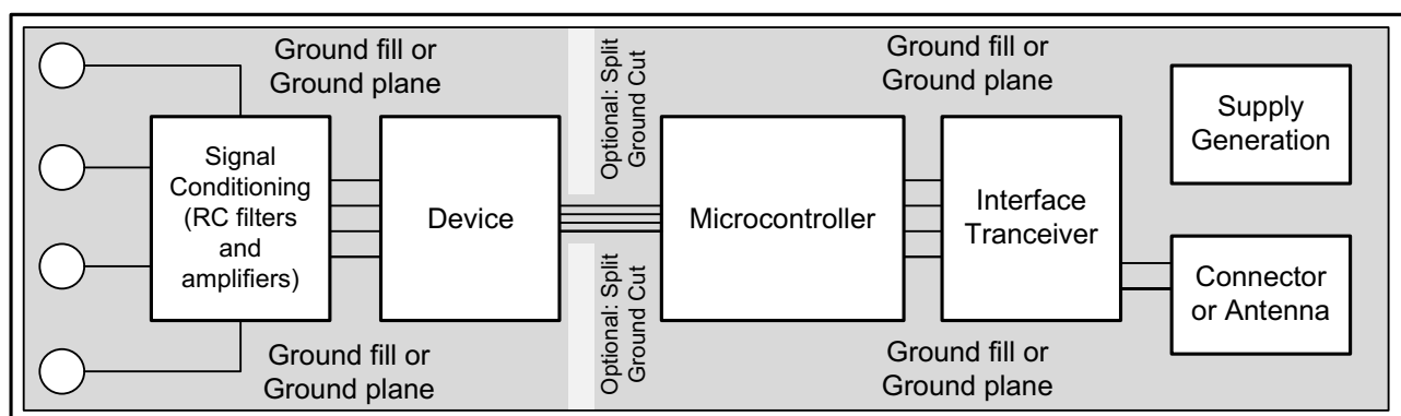
Figure 85. System Component Placement
