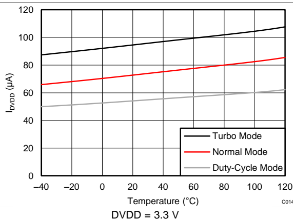
Figure 35. I_{DVDD} vs Temperature
