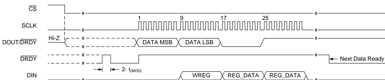
Figure 66. Example of Reading Data while Simultaneously Sending a WREG Command
