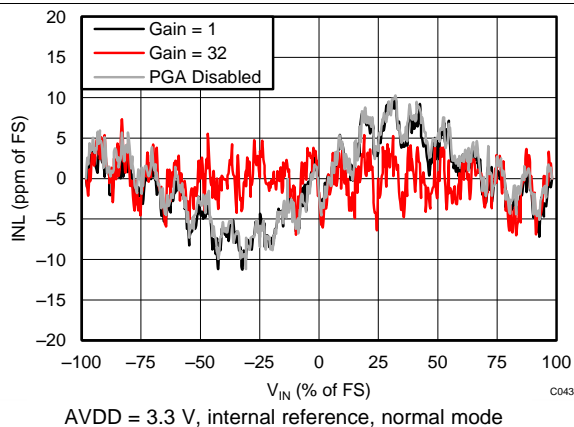
Figure 9. Integral Nonlinearity vs Differential Input Signal
