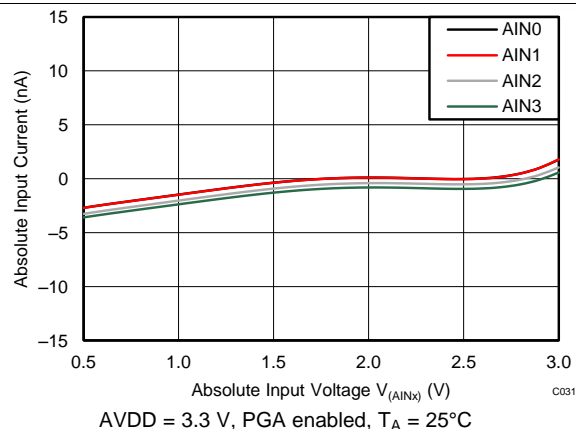
Figure 16. Absolute Input Current vs Absolute Input Voltage
