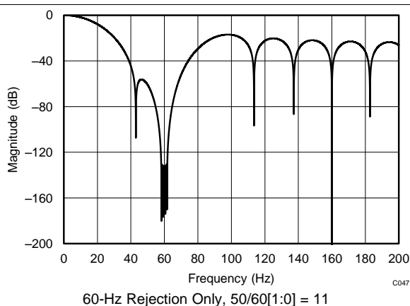
Figure 50. Filter Response (DR = 20 SPS)
