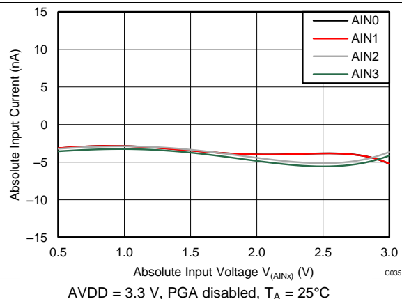
Figure 22. Absolute Input Current vs Absolute Input Voltage
