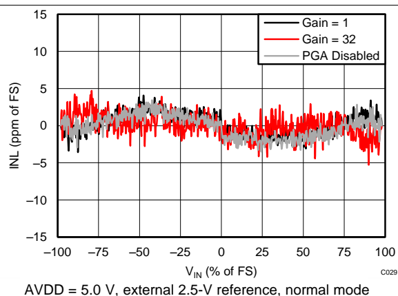
Figure 8. Integral Nonlinearity vs Differential Input Signal
