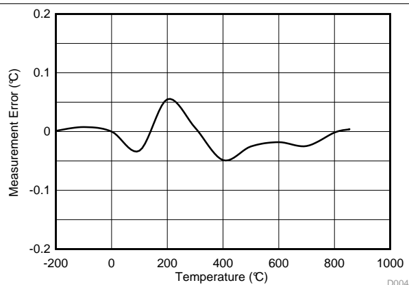
Figure 81. Temperature Measurement Error vs T_{(RTD)}
