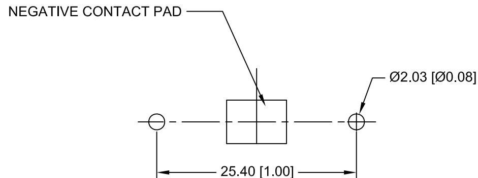
PCB LAYOUT
