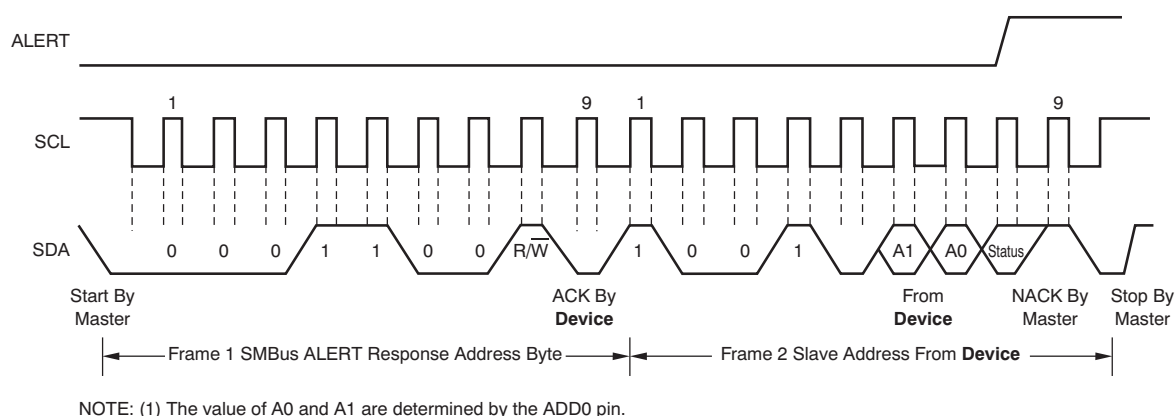
Figure 11. Timing Diagram for SMBus ALERT
