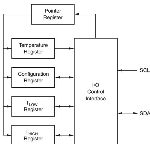
Figure 13. Internal Register Structure
