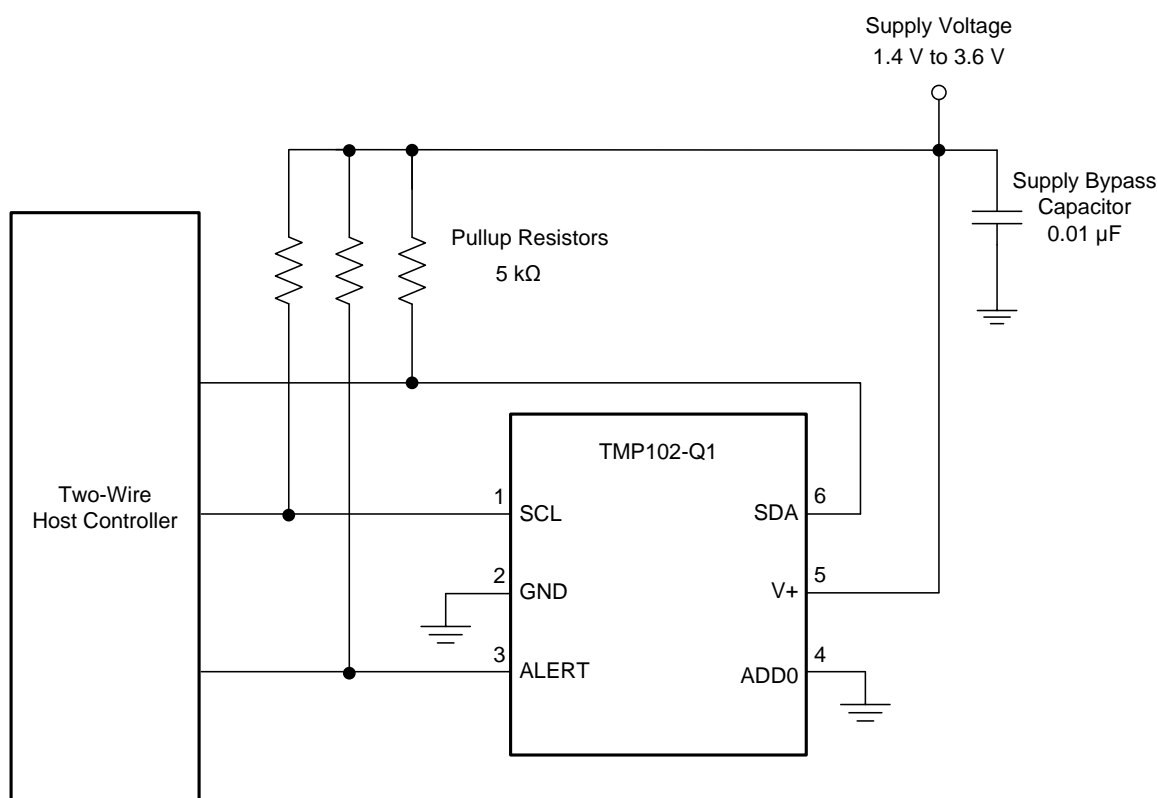
Figure 15. Typical Connections
