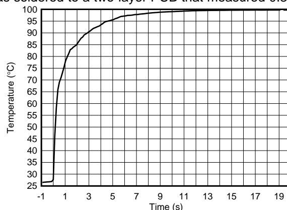
Figure 17. Temperature Step Response
