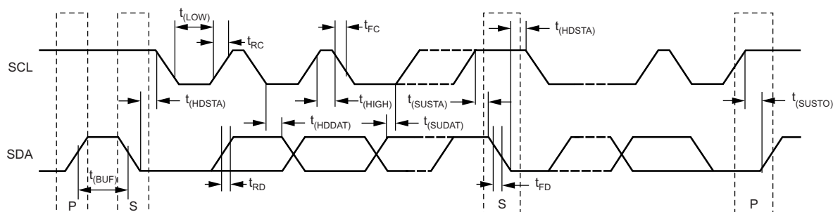
Figure 8. Two-Wire Timing Diagram
