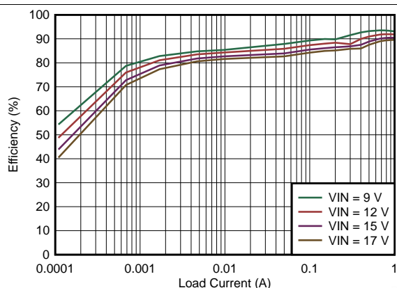
Figure 70. Efficiency V_{OUT} = 5.0\text{ V}
