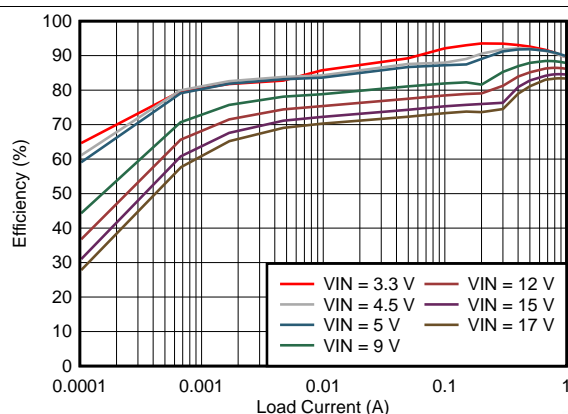
Figure 46. Efficiency V_{OUT} = 2.5\text{ V}
