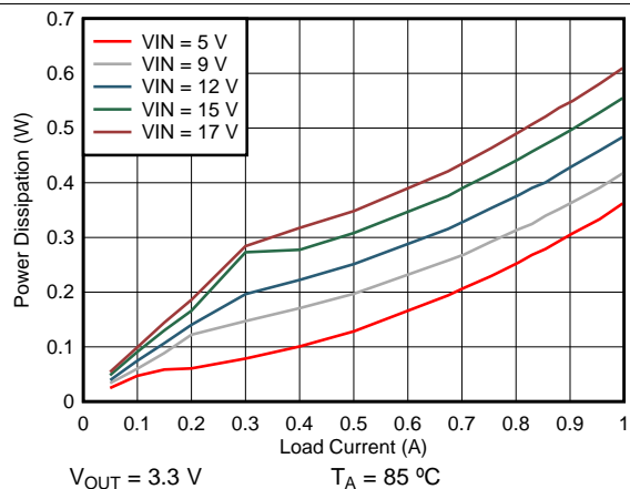
Figure 6. Power Dissipation
