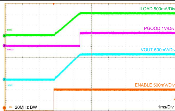
Figure 25. Startup V_{OUT} = 1.2\text{ V}
