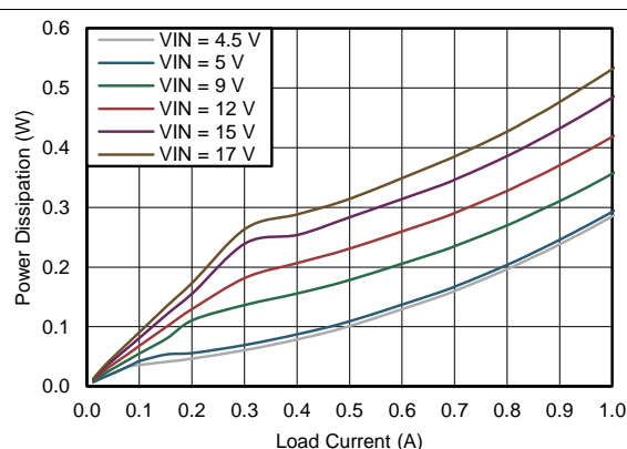
Figure 59. Power Dissipation V_{OUT} = 3.3\text{ V}
