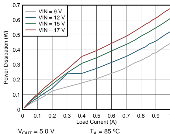
Figure 7. Power Dissipation
