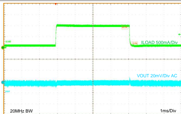
Figure 36. Load Transient V_{OUT} = 1.8\text{ V}
