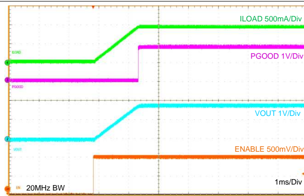
Figure 37. Startup V_{OUT} = 1.8\text{ V}
