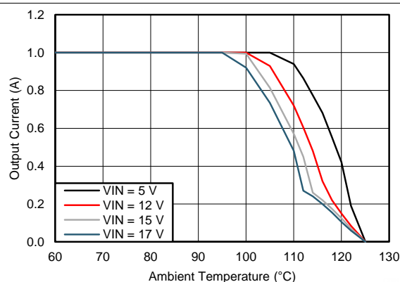
Figure 55. Thermal Derating for \theta_{JA} = 47^\circ\text{C/W} , V_{OUT} = 2.5\text{ V}
