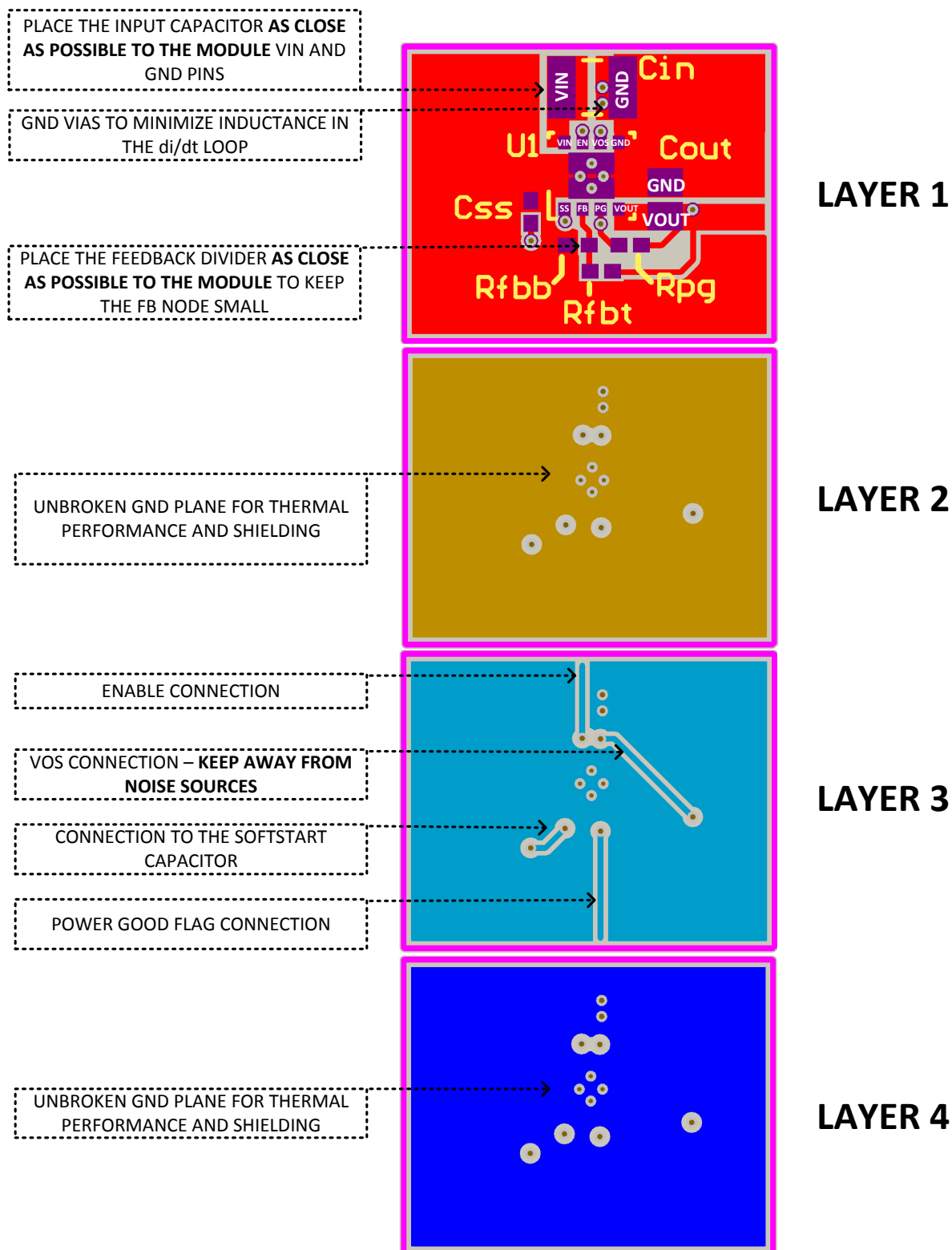
Figure 81. Layout example
