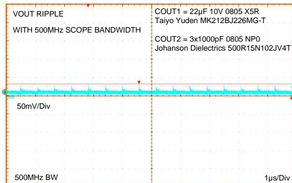
Figure 27. 500 MHz Oscilloscope Bandwidth, 3x1000 pF additional output capacitance Output Voltage Ripple and HF Noise V_{OUT} = 1.2\text{ V}
