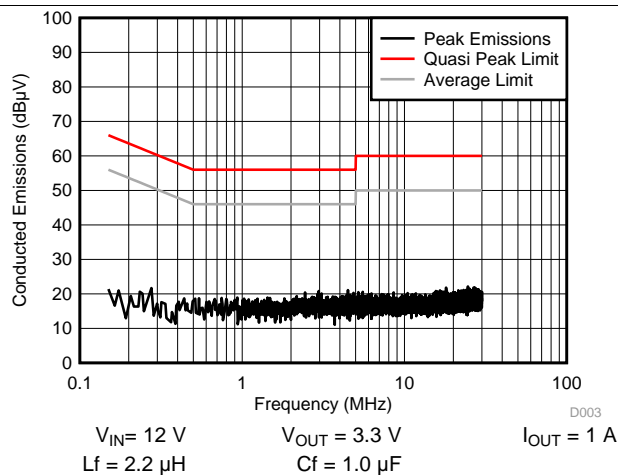
Figure 11. Conducted EMI on EVM
