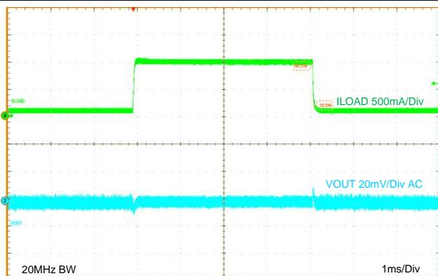
Figure 48. Load Transient V_{OUT} = 2.5\text{ V}
