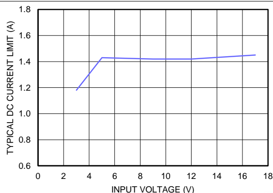
Figure 53. Typical Current Limit V_{OUT} = 2.5\text{ V} , T_A = 85^\circ\text{C}
