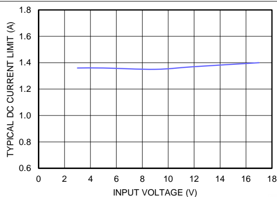
Figure 41. Typical Current Limit V_{OUT} = 1.8 V, T_A = 85^\circ\text{C}
