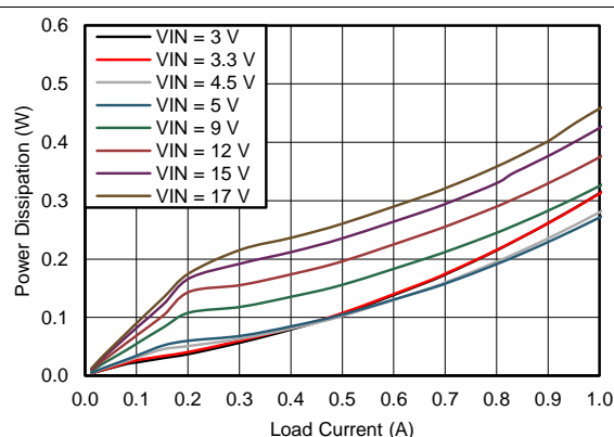
Figure 35. Power Dissipation V_{OUT} = 1.8\text{ V}
