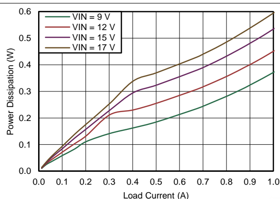
Figure 71. Power Dissipation V_{OUT} = 5.0\text{ V}
