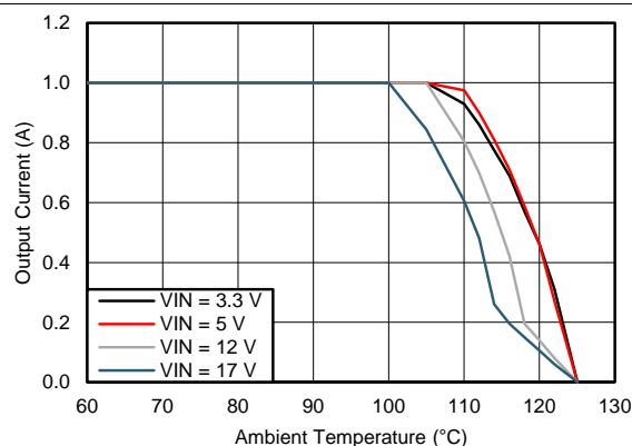
Figure 43. Thermal Derating for \theta_{JA} = 47^\circ\text{C/W} V_{OUT} = 1.8 V
