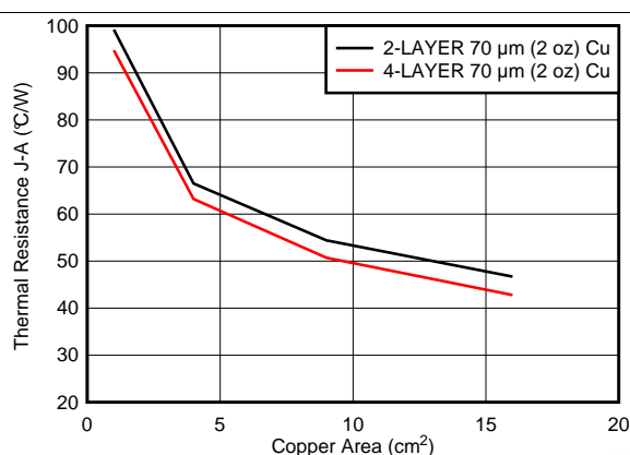
Figure 2. Package Thermal Resistance vs. Board Copper Area
