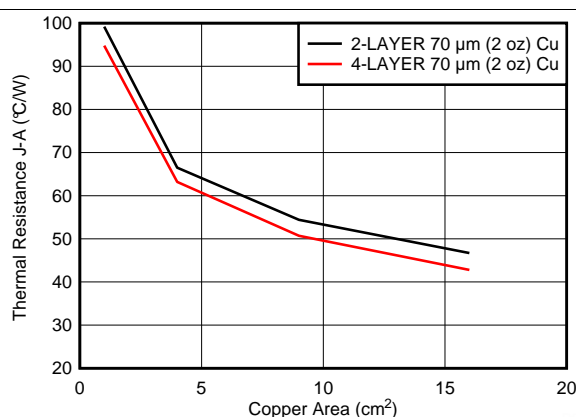
Figure 80. Package Thermal Resistance vs. Board Copper Area
