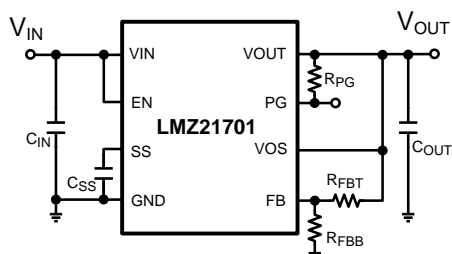
Figure 14. Typical Applications Circuit
