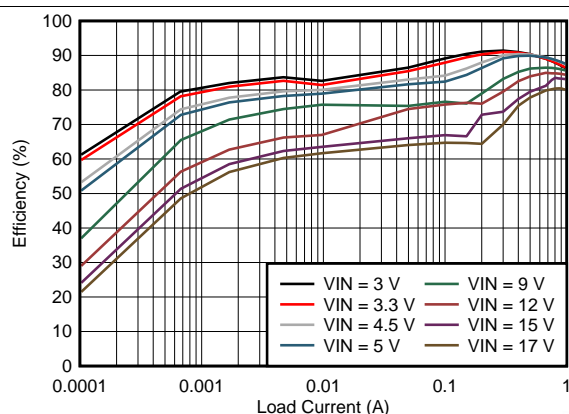
Figure 34. Efficiency V_{OUT} = 1.8\text{ V}
