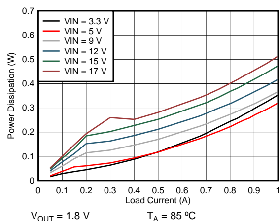
Figure 4. Power Dissipation
