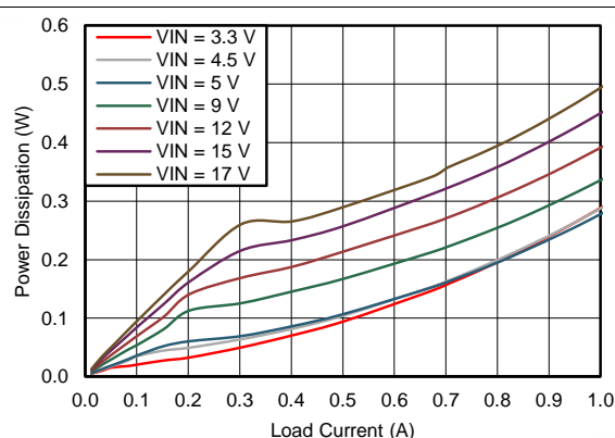
Figure 47. Power Dissipation V_{OUT} = 2.5\text{ V}
