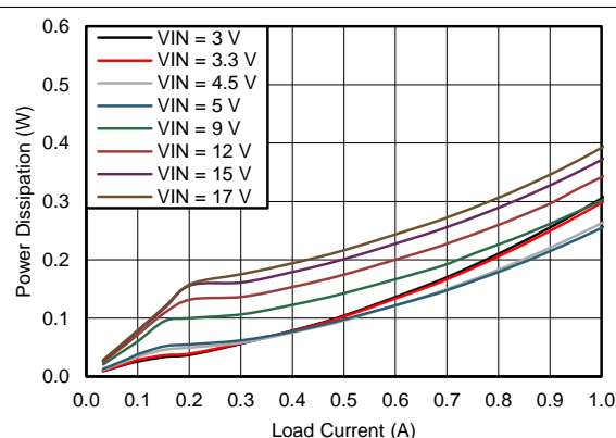
Figure 23. Power Dissipation V_{OUT} = 1.2\text{ V}
