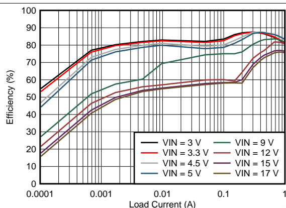
Figure 22. Efficiency V_{OUT} = 1.2\text{ V}
