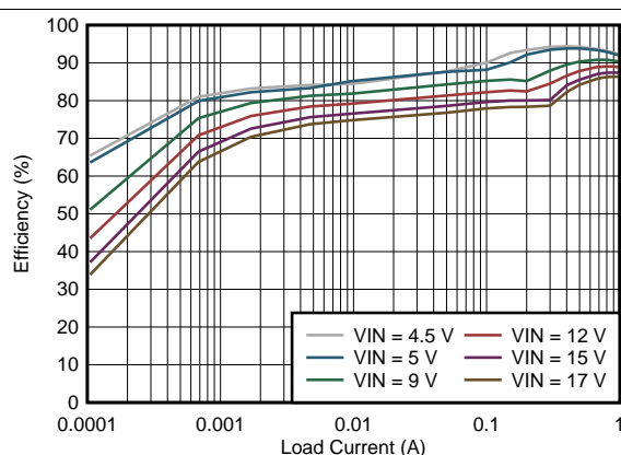
Figure 58. Efficiency V_{OUT} = 3.3\text{ V}
