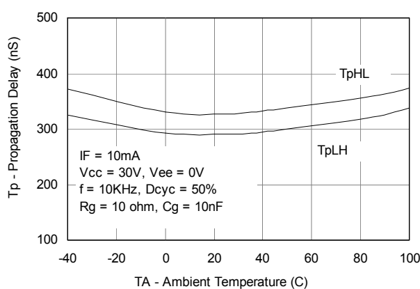
Figure 12: Propagation vs Temperature
