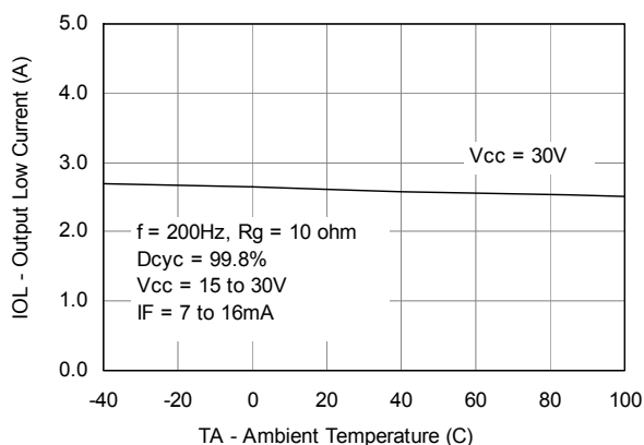
Figure 5: Output Low Current vs Temperature Current
