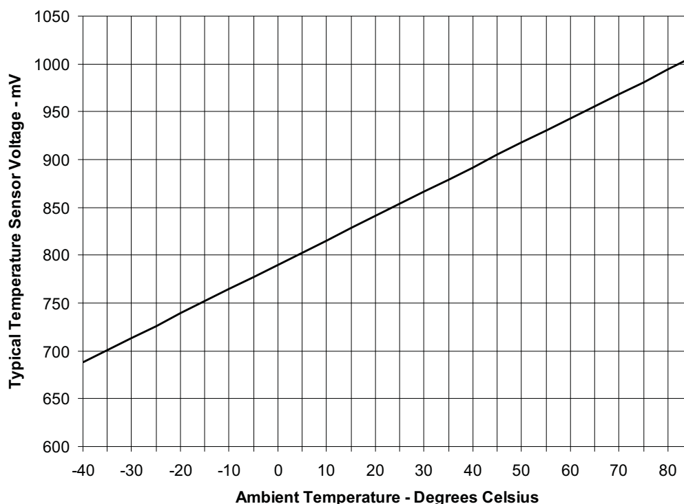
Figure 4-11. Typical Temperature Sensor Voltage
