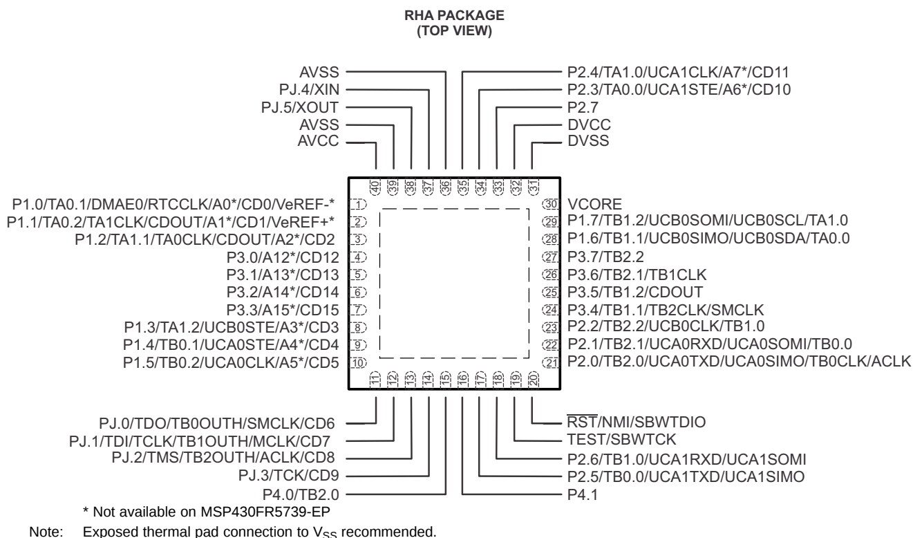
Figure 3-1. 40-Pin RHA Package (Top View)
