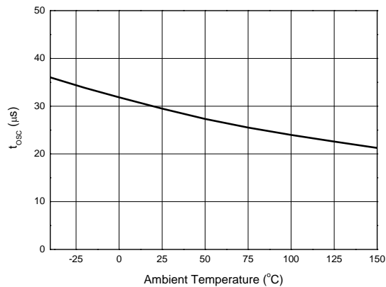
Oscillation Period vs. Ambient Temperature
