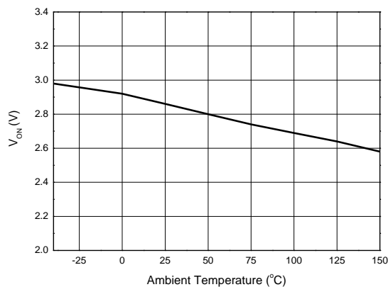
Power-on Voltage vs. Ambient Temperature
