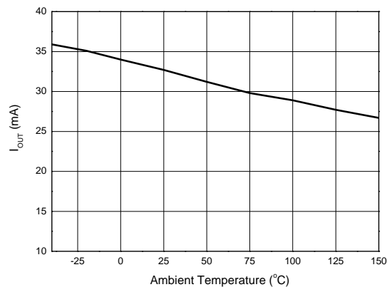
Output Current vs. Ambient Temperature
