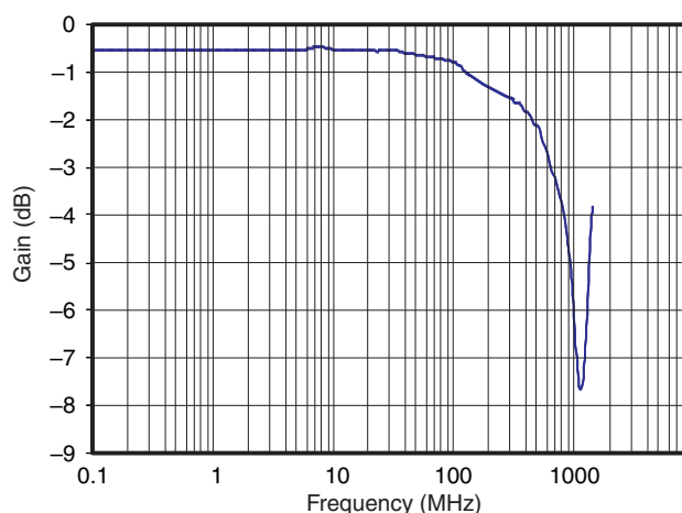
Figure 10. 3-dB Bandwidth
