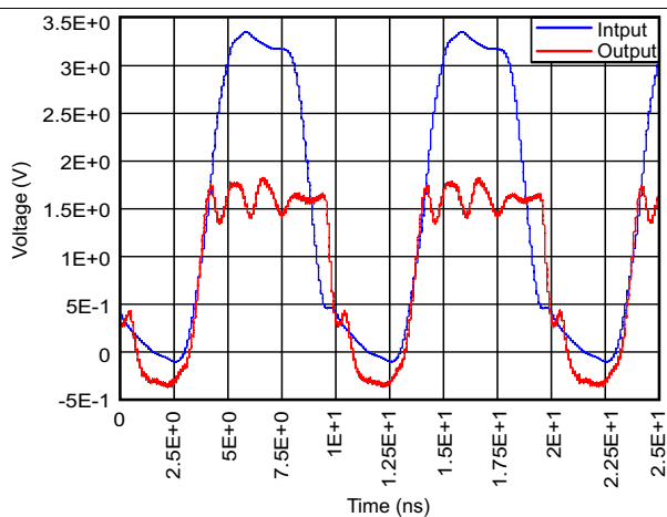
Figure 17. Waveform From TP1 (Pullup Resistor: 160-Ω and 50-pF Capacitance 3.3 to 1.8 V at 100 MHz)
