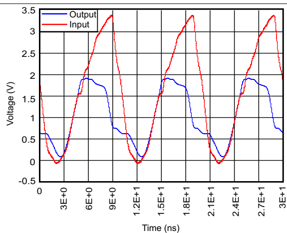
Figure 18. Waveform From TP2 (Pullup Resistor: 160-Ω and 50-pF Capacitance 1.8 to 3.3 V at 100 MHz)
