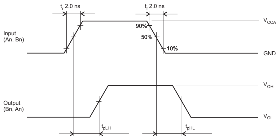
Figure 7. t_{PLH} , t_{PHL}
