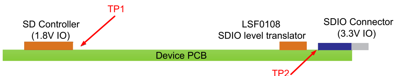
Figure 16. Device Placement
