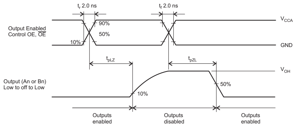
Figure 8. t_{PLZ} , t_{PZL}
