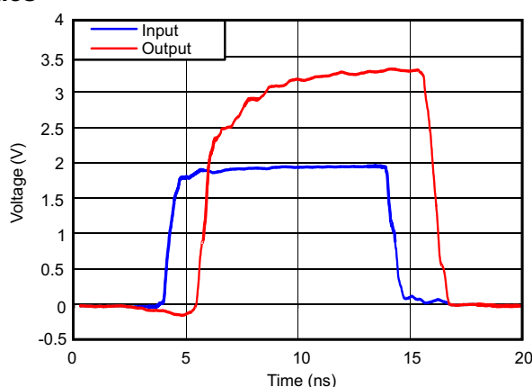
Figure 4. Signal Integrity (1.8 V to 3.3 V Translation Up at 50 MHz)
