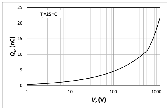
Fig. 6 Recovery Charge
