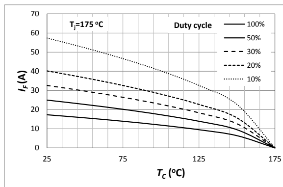
Fig. 4 Current Derating
