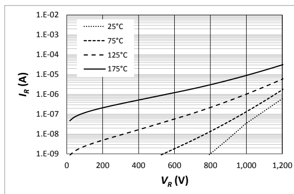
Fig. 2 Reverse Characteristics (parameterized on T_J )
