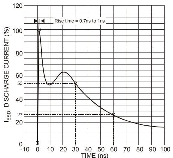
Figure 2 ESD Discharge Current Wave Form IEC 6100-4-2 (330Ω/150pF)
