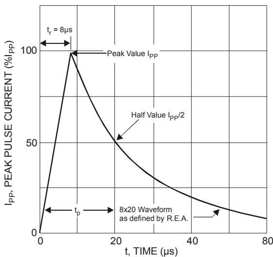
Figure 1 Pulse Waveform
