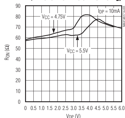
DP/DM SHORT ON-RESISTANCE vs. VDP
