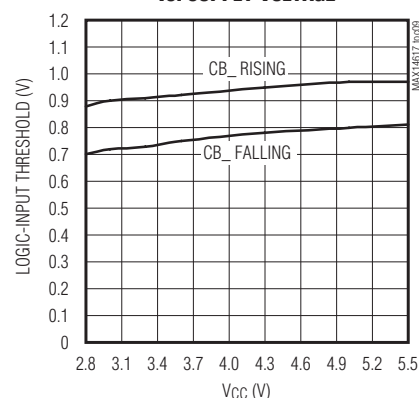
LOGIC-INPUT THRESHOLD vs. SUPPLY VOLTAGE
