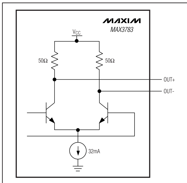
Figure 2. CML Output Structure
