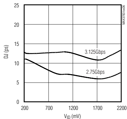
DETERMINISTIC JITTER vs. CML DIFFERENTIAL INPUT VOLTAGE
