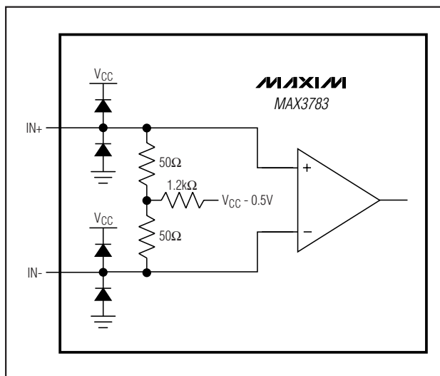
Figure 1. Input Structure
