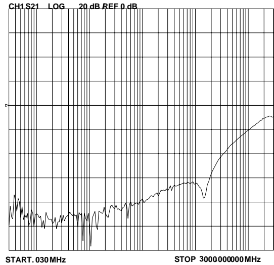
Analog Crosstalk
