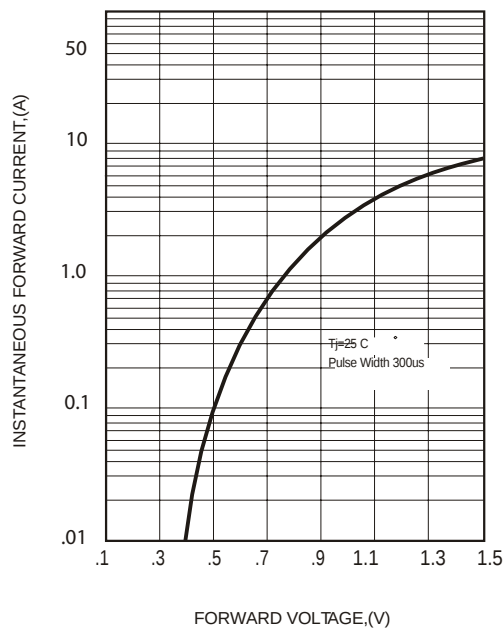
FIG.2-TYPICAL FORWARD CHARACTERISTICS
