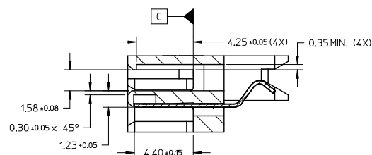
SECTION T-T
