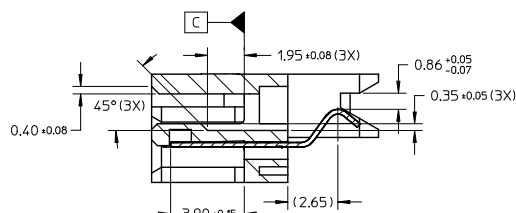
SECTION U-U
