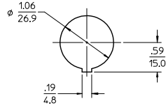
PANEL CUTOUT SCALE: 1:1
