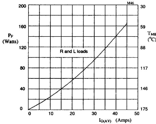
Figure 6. Forward power dissipation and maximum allowable mounting base temperature as a function of output current for sinusoidal operation, for SET111403 and SET111412.
