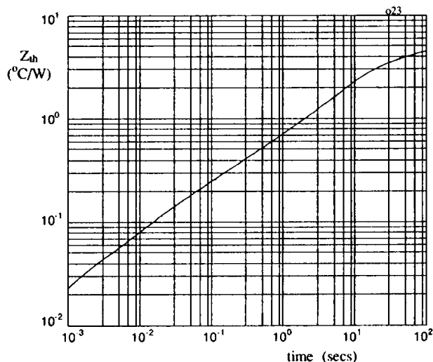
Fig 2. Transient thermal impedance characteristic per leg
